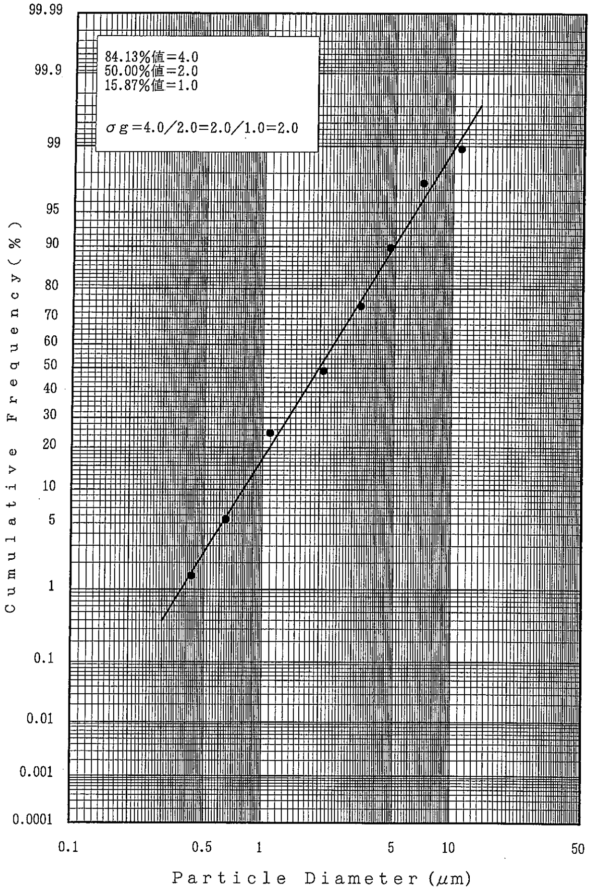
FIGURE 6 PARTICLE SIZE DISTRIBUTION CURVE [ 1 mg/m 3 : FOURTH WEEK ]
