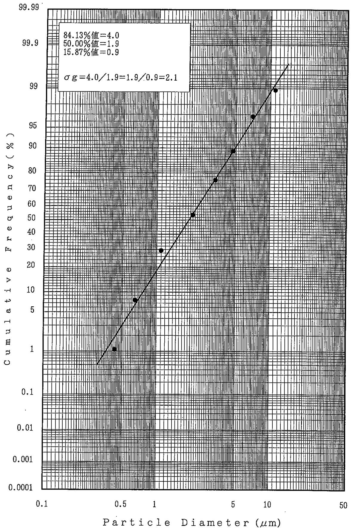
FIGURE 14 PARTICLE SIZE DISTRIBUTION CURVE [ 10 mg/m 3 : FOURTH WEEK ]
