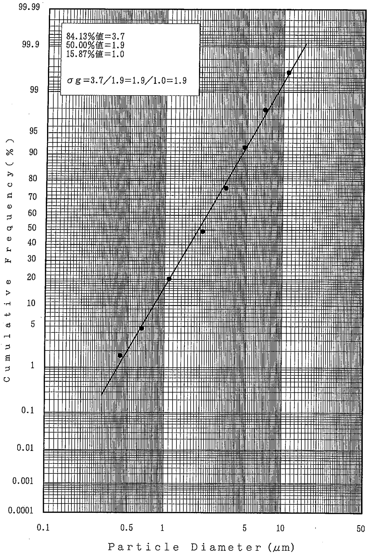
FIGURE 8 PARTICLE SIZE DISTRIBUTION CURVE [ 3 mg/m 3 : SECOND WEEK ]
