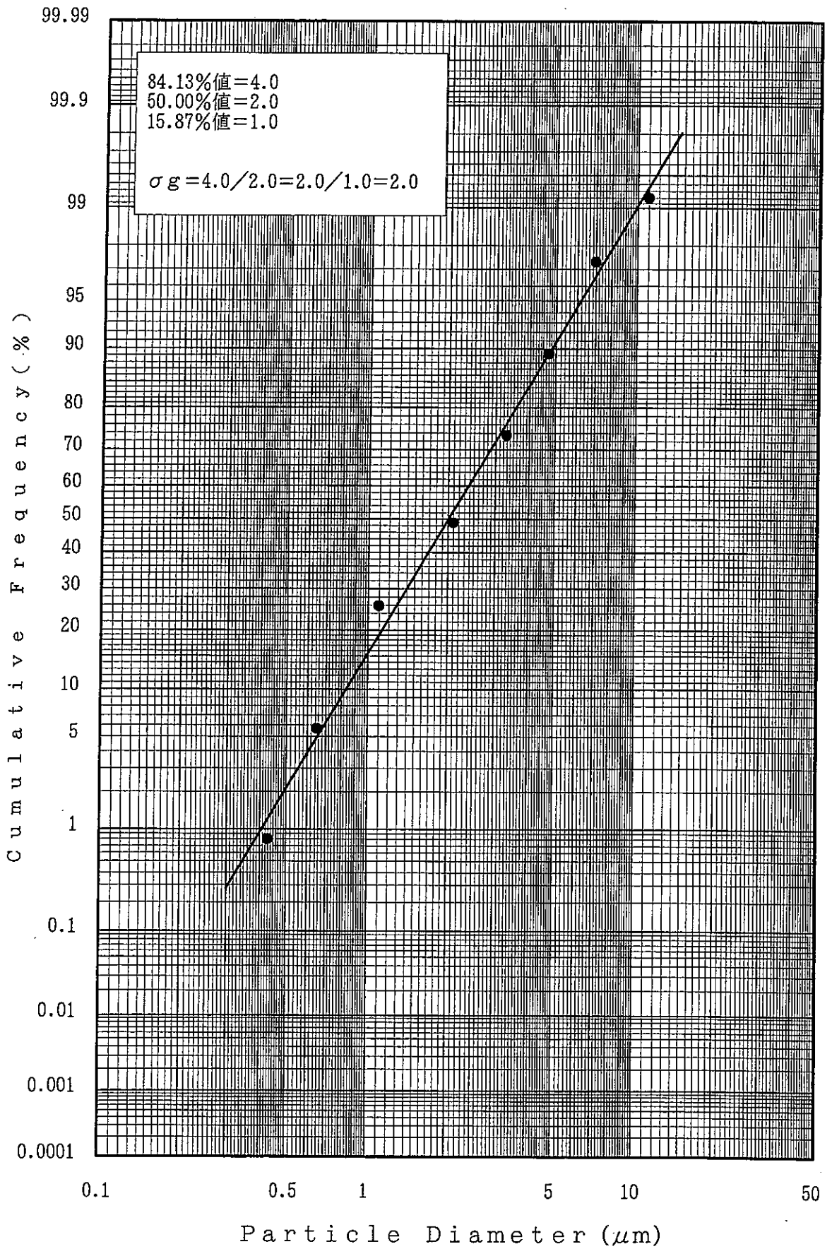
FIGURE 4 PARTICLE SIZE DISTRIBUTION CURVE [ 1 mg/m 3 : SECOND WEEK ]
