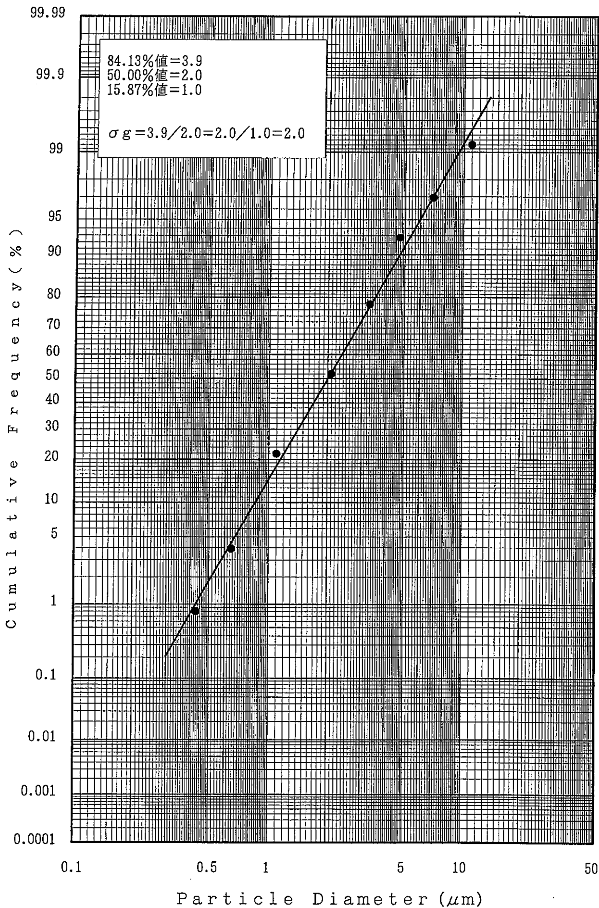
FIGURE 9 PARTICLE SIZE DISTRIBUTION CURVE [ 3 mg/m 3 : THIRD WEEK ]
