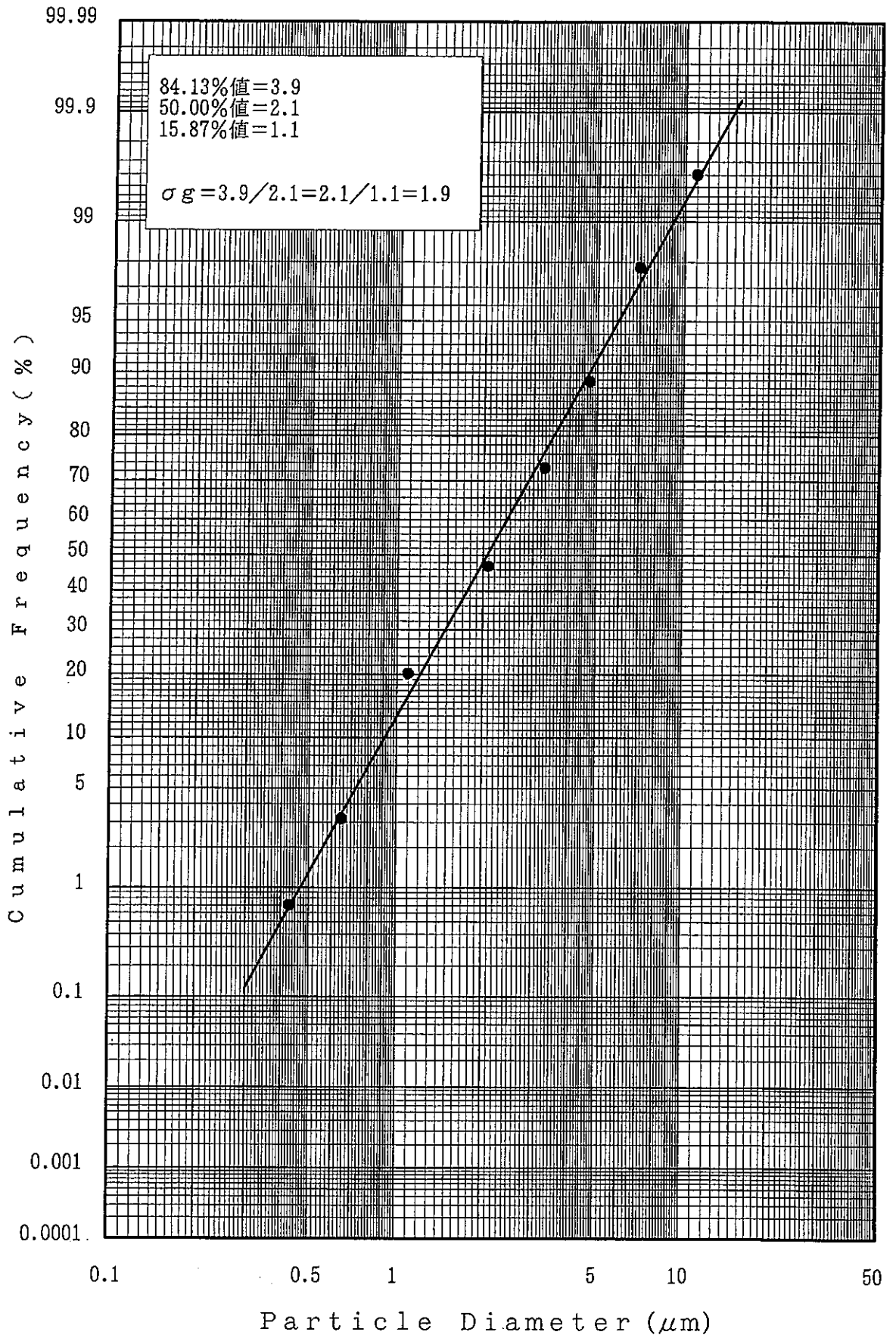
FIGURE 3 PARTICLE SIZE DISTRIBUTION CURVE [ 1 mg/m 3 : FIRST WEEK ]
