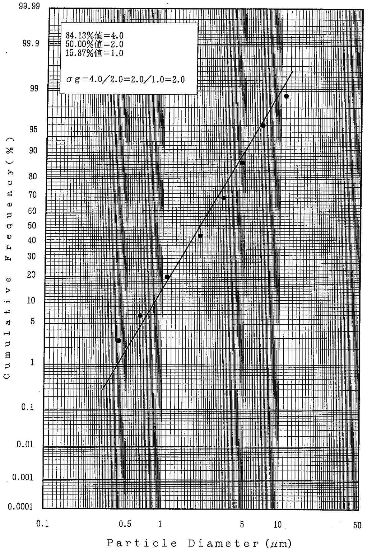
FIGURE 5 PARTICLE SIZE DISTRIBUTION CURVE [ 1 mg/m 3 : THIRD WEEK ]
