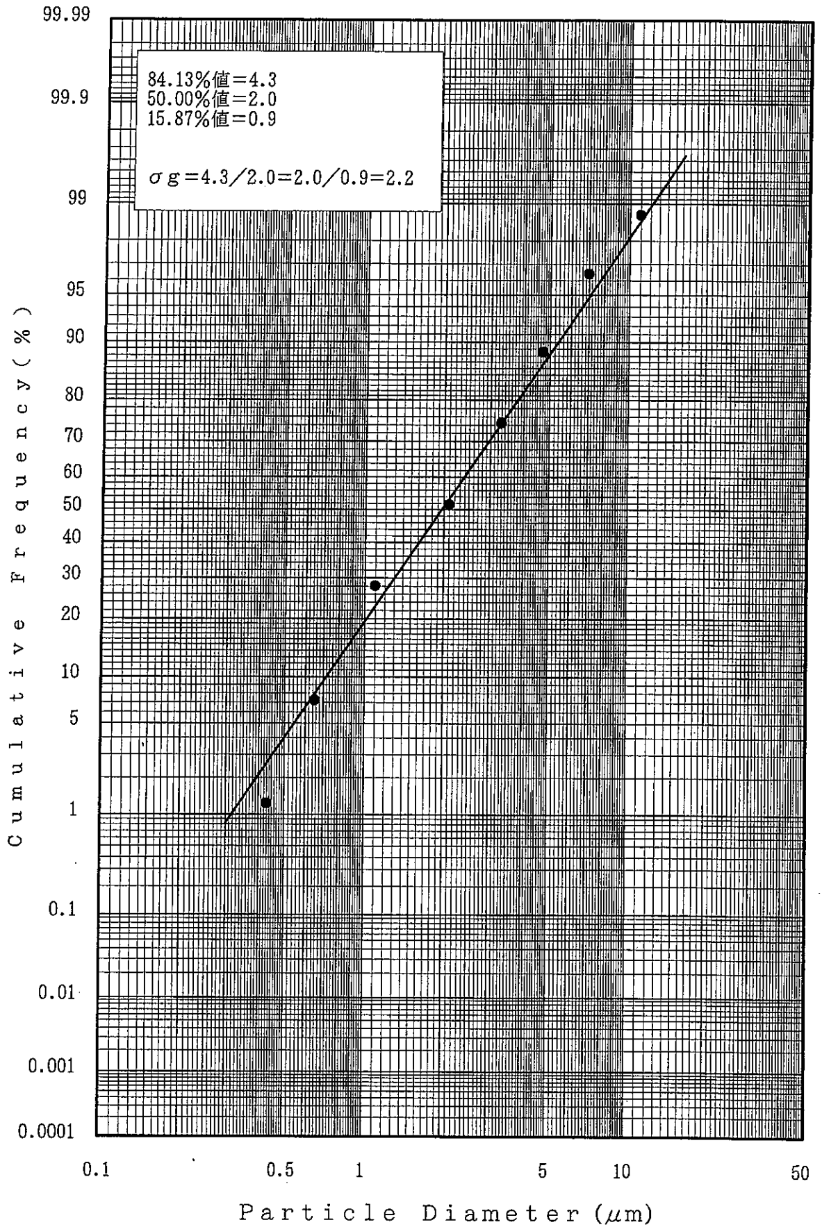
FIGURE 11 PARTICLE SIZE DISTRIBUTION CURVE [ 10 mg/m 3 : FIRST WEEK ]
