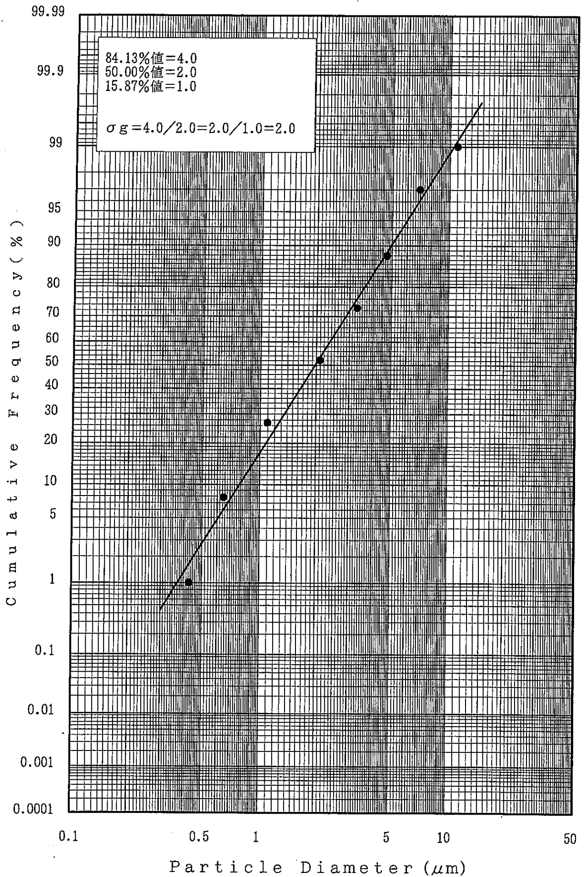
FIGURE 13 PARTICLE SIZE DISTRIBUTION CURVE [ 10 mg/m 3 : THIRD WEEK ]
