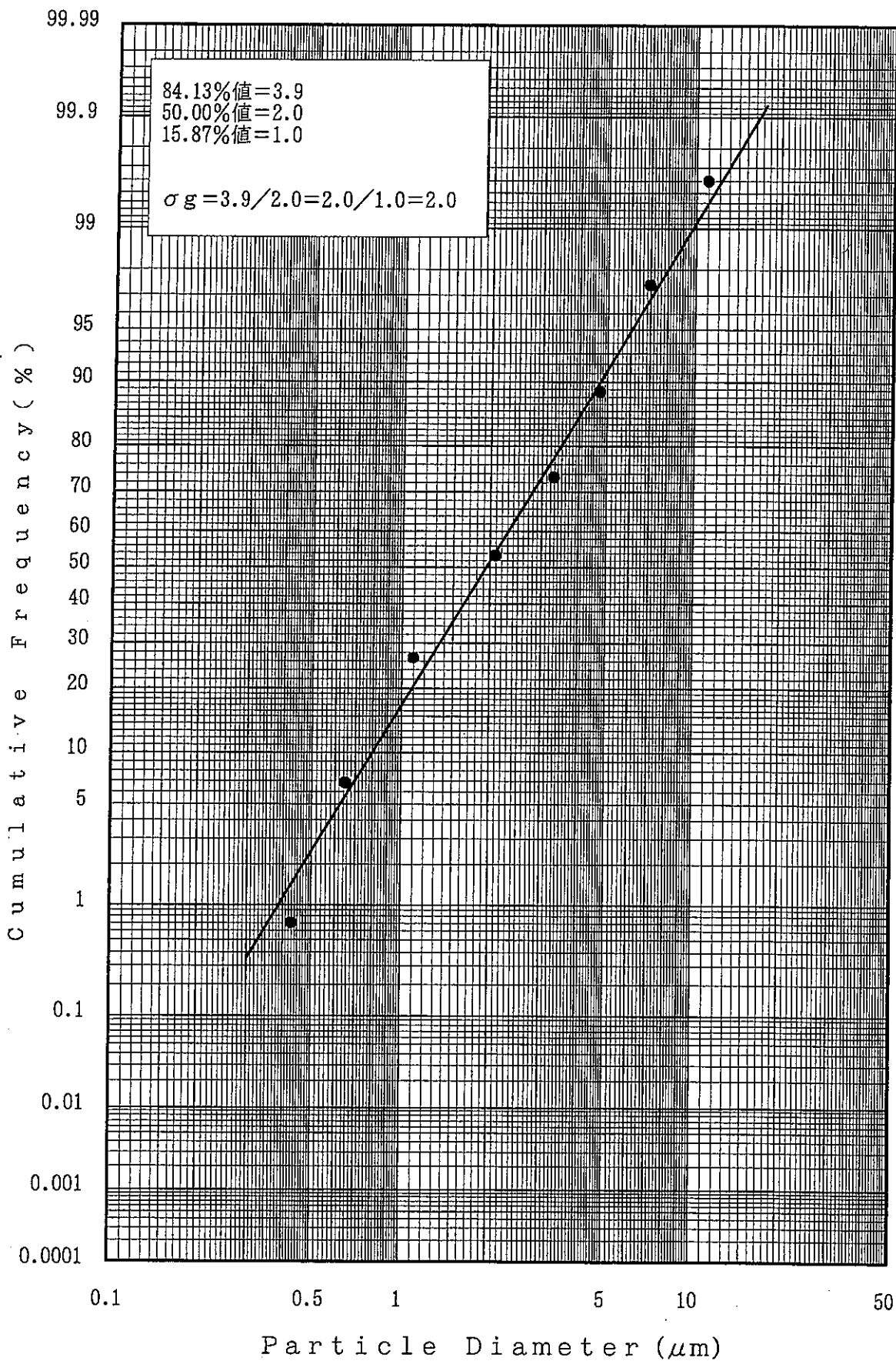
FIGURE 12 PARTICLE SIZE DISTRIBUTION CURVE [ 10 mg/m 3 : SECOND WEEK ]
