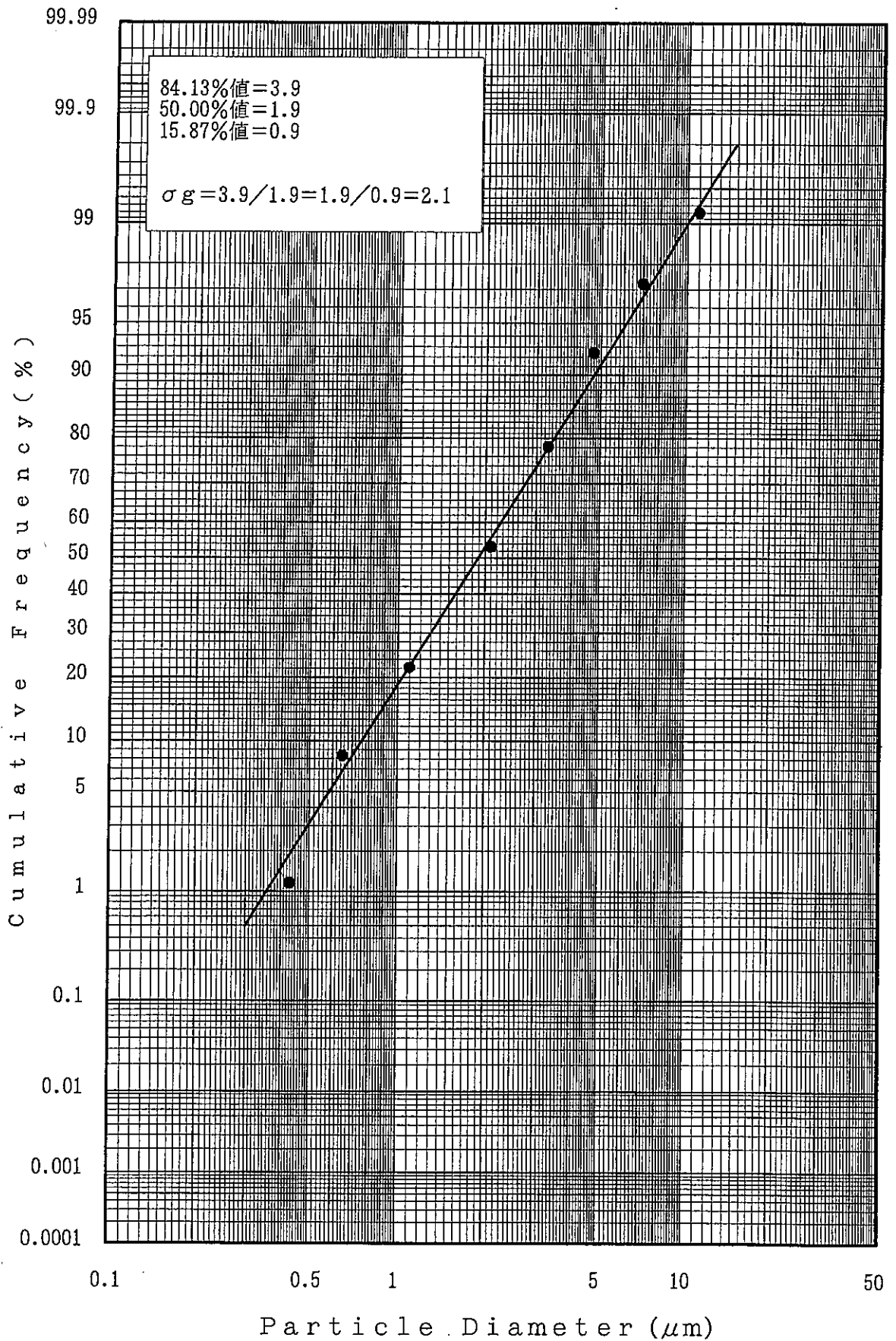
FIGURE 10 PARTICLE SIZE DISTRIBUTION CURVE [ 3 mg/m 3 : FOURTH WEEK ]
