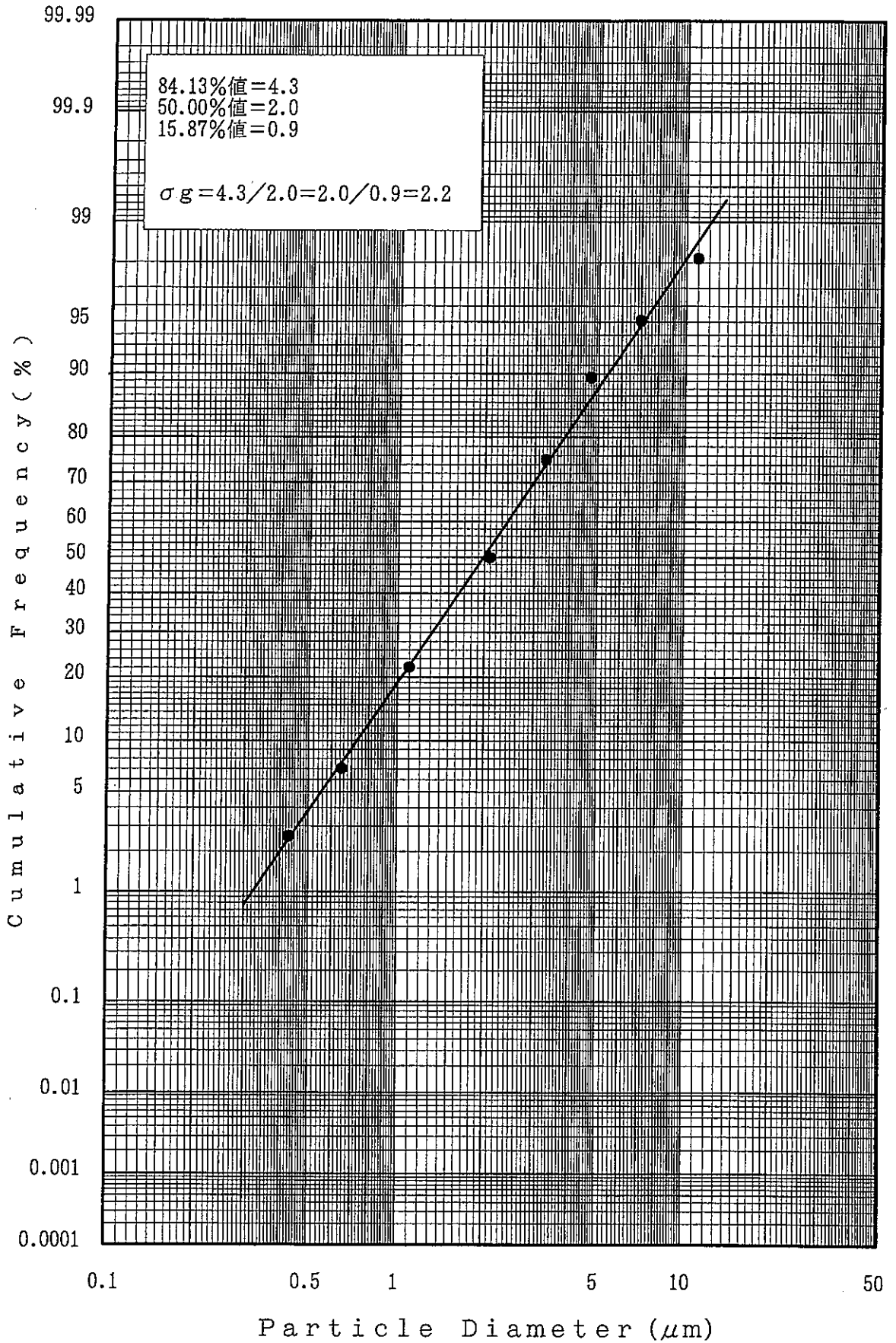
FIGURE 7 PARTICLE SIZE DISTRIBUTION CURVE [ 3 mg/m 3 : FIRST WEEK ]
