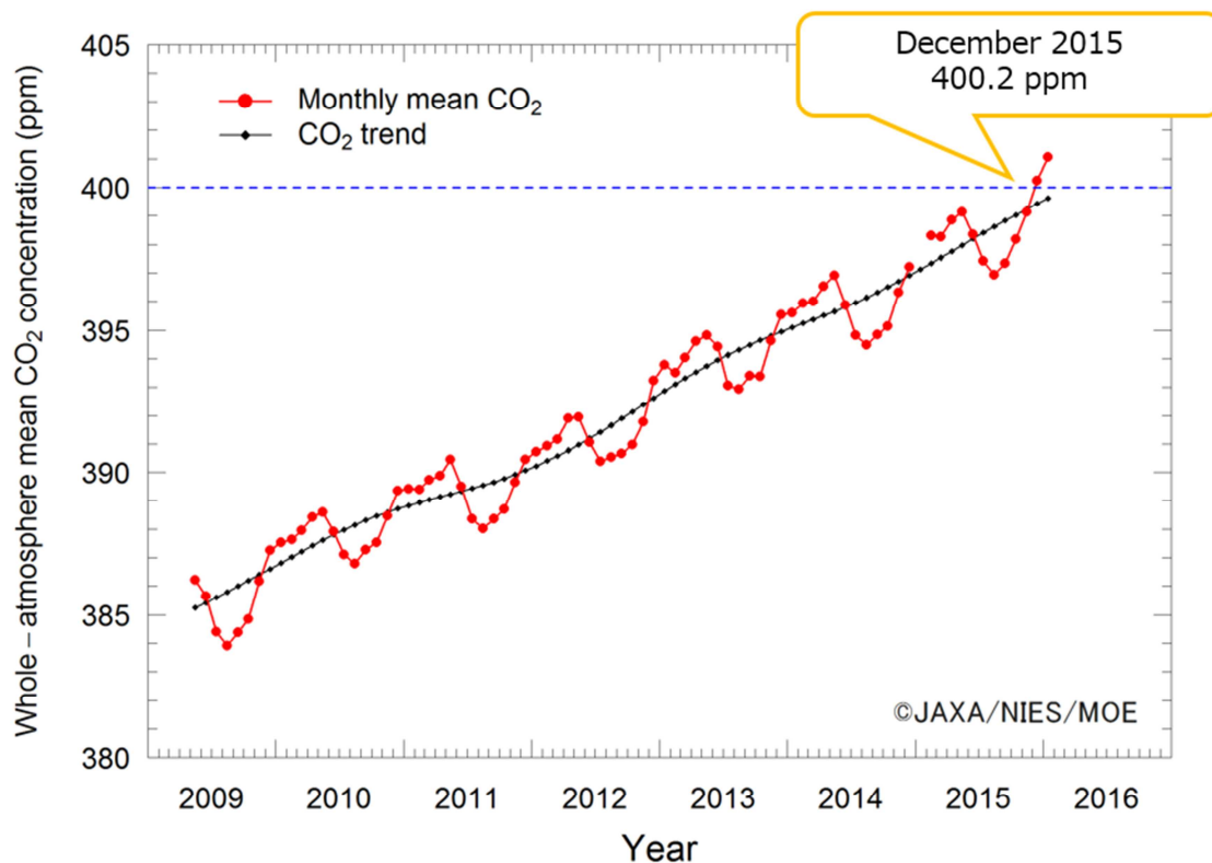
Whole-atmospheric CO 2 concentrations monitored by GOSAT: monthly mean (●) and trend (●).
