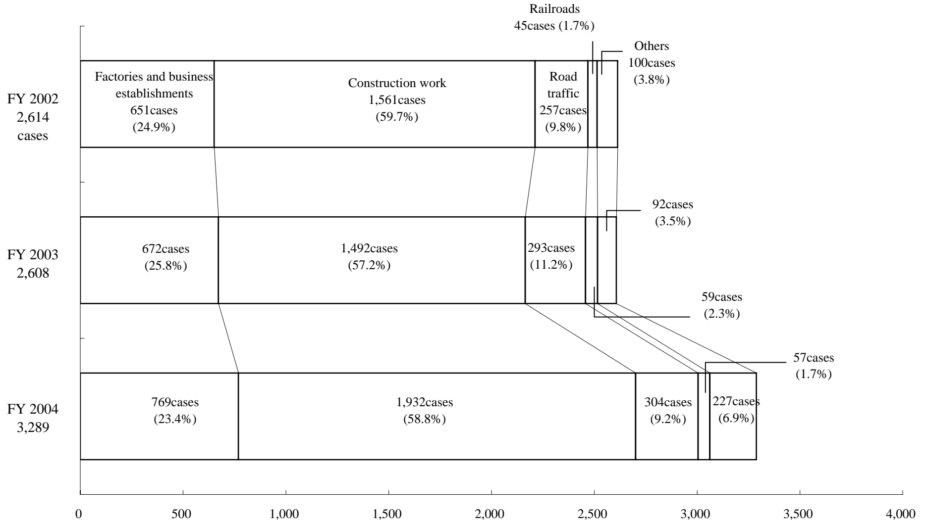
Fig. 3 Changes in the Number of Complaints about Vibration by Source (FY 2002 - FY 2004)
