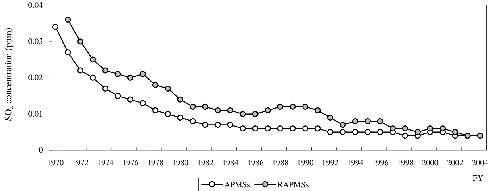
Fig. 4-2 Changes in Annual Average Concentration of Sulfur Dioxide
