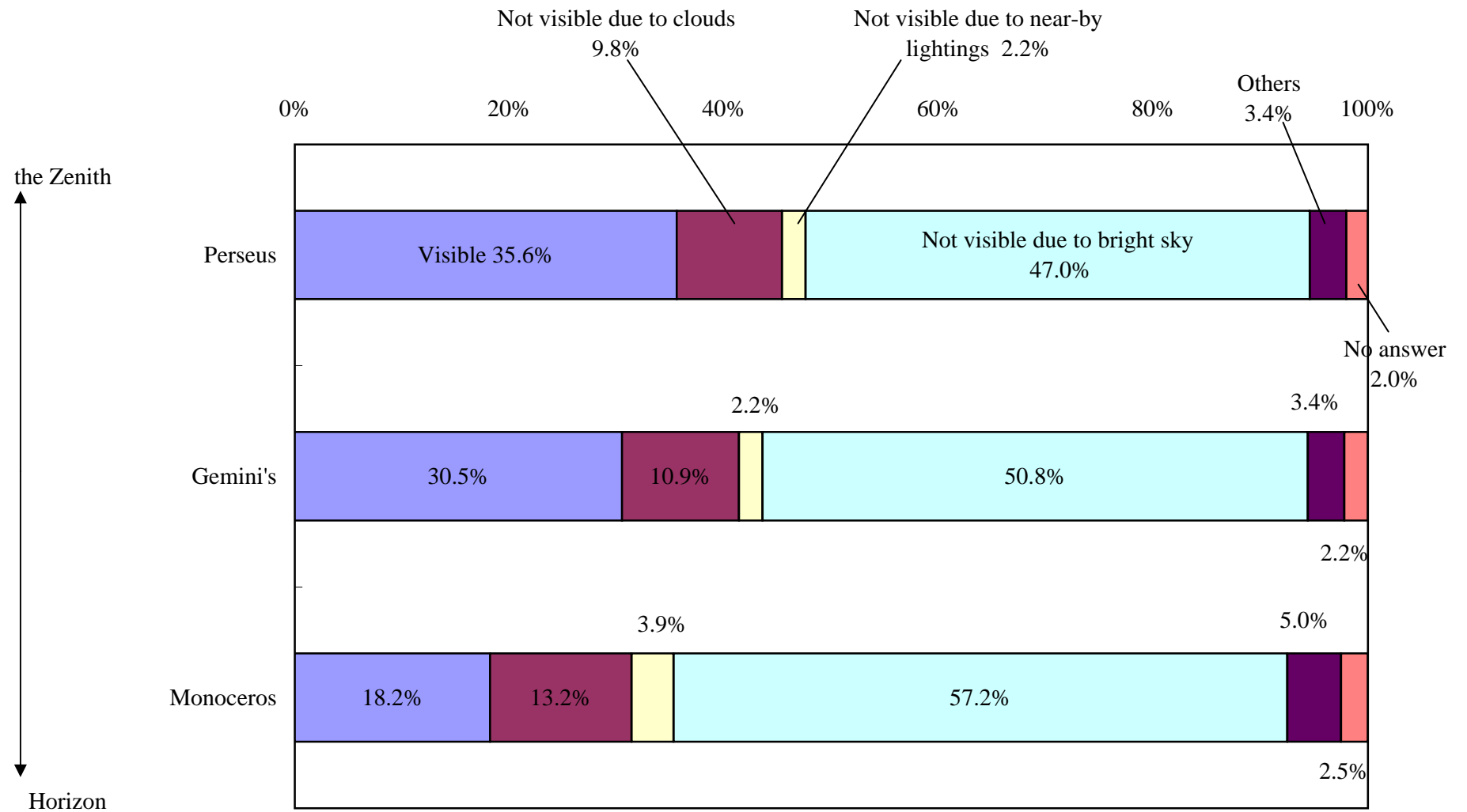
Fig. 1 Naked Eye Observation Result of the Milky Way (Winter, 2004)
