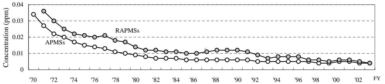
Fig.4-2 Changes in Annual Average Concentration of Sulfur Dioxide
