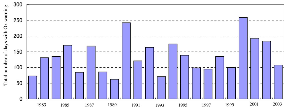
Fig.3-2 Changes in Number of Days of Photochemical Oxidant (Ox) Warning Issued
