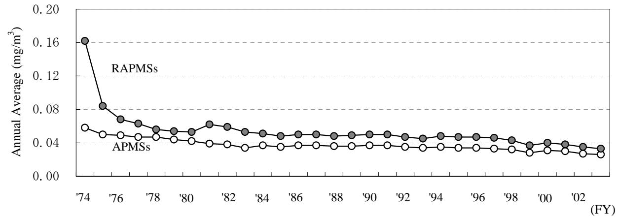
Fig. 2-2 Changes in Annual Average Concentration of Suspended Particulate Matter
