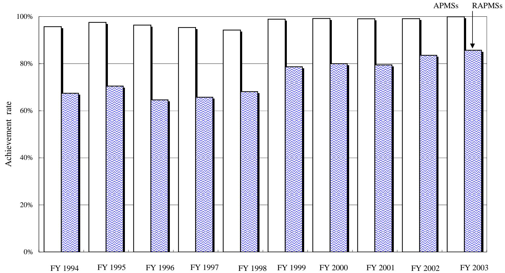
Fig. 1-1 Changes in Achievement Rate of Environmental Quality Standard for Nitrogen Dioxide
