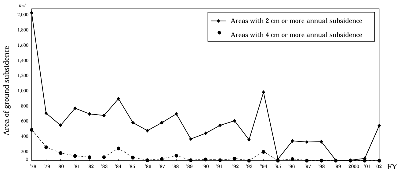
Fig.2 Total Area of Ground Subsidence in Japan (Changes by Fiscal Year)
