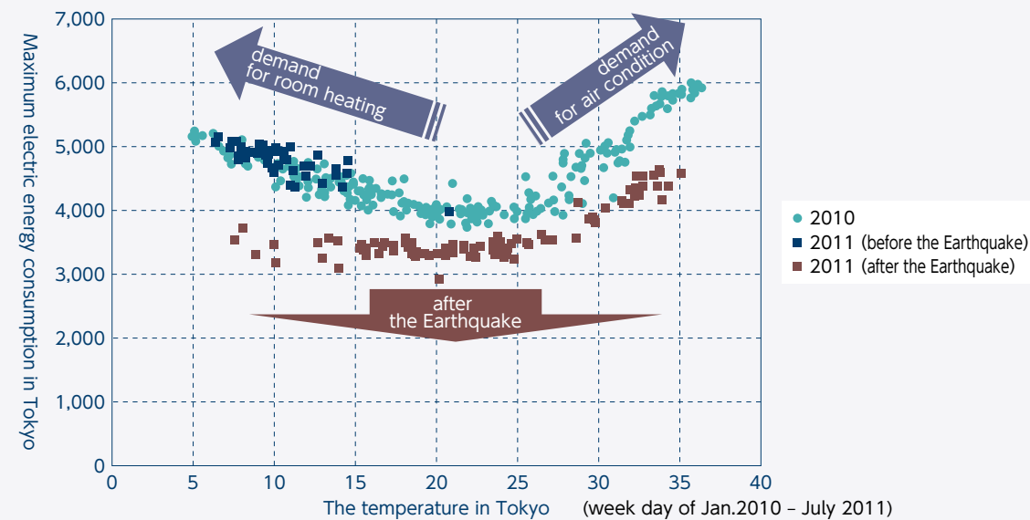
Figure 2-2-1 Relationship between the Temperature and Electric Consumption of TEPCO Area in 2010 and 2011
