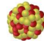
Radium-226 { 88 protons 138 neutrons }
