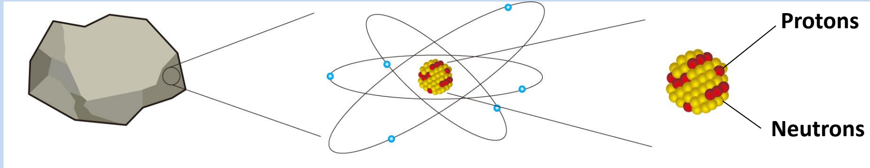
\alpha -particles { Two protons Two neutrons }
