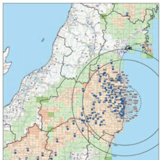
Deposition Amount of Sr-90 (as of Jan. 13, 2012)
