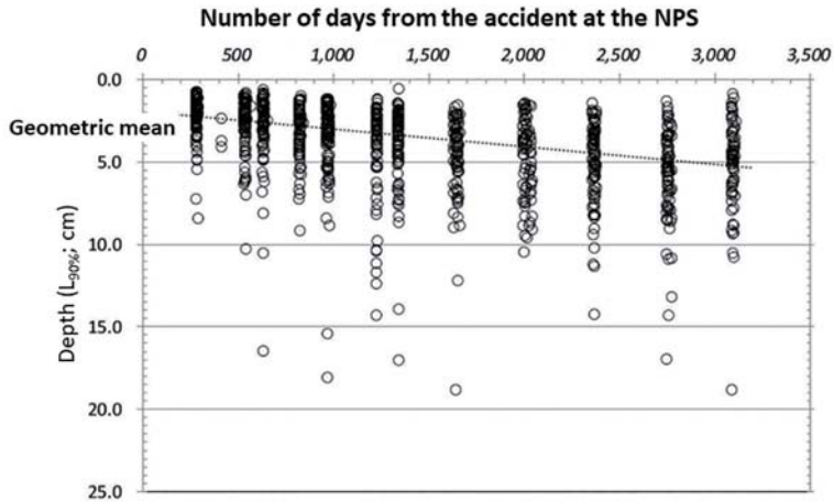
Figure: Data on changes over time in L 90% since December 2011 (85 locations at uncultivated land in Fukushima Prefecture, the southern part of Miyagi Prefecture and the northern part of Ibaraki Prefecture) (Reference) Depth (L 90% ): The depth from the ground surface where 90% of all deposited radioactive cesium is contained Source: Prepared based on the outcome report, "Survey of Depth Distribution of Radioactive Cesium in Soil," of the FY2019 project, "Compilation of Data on Distribution of Radioactive Materials Released due to the Accident at Tokyo Electric Power Company (TEPCO)'s Fukushima Daiichi NPS" commissioned by the Secretariat of the Nuclear Regulation Authority
