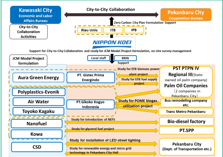
Implementation Structure
