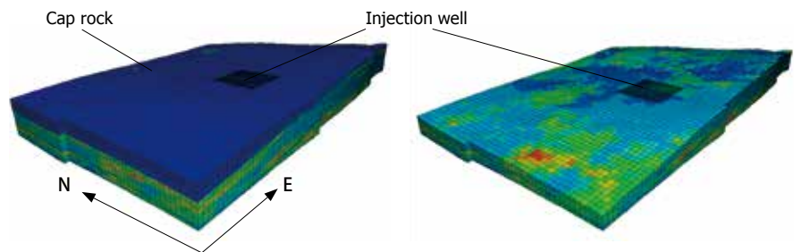
Modeling of permeability distribution of the sub-sea reservoir (10km×8km area in this case). Numerical simulations using this model are conducted to estimate the dynamics of CO 2 under the cap rock. Illustrated by Taisei Corporation
