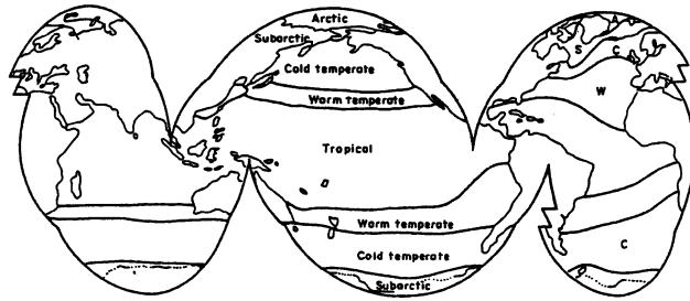
Climatic regions
