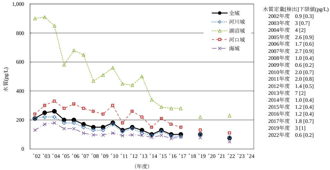
[11-2] \beta -HCH
