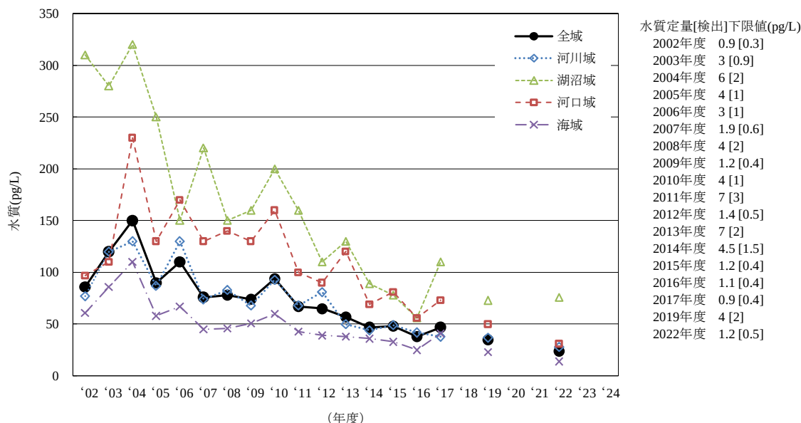
[11-1] \alpha -HCH
