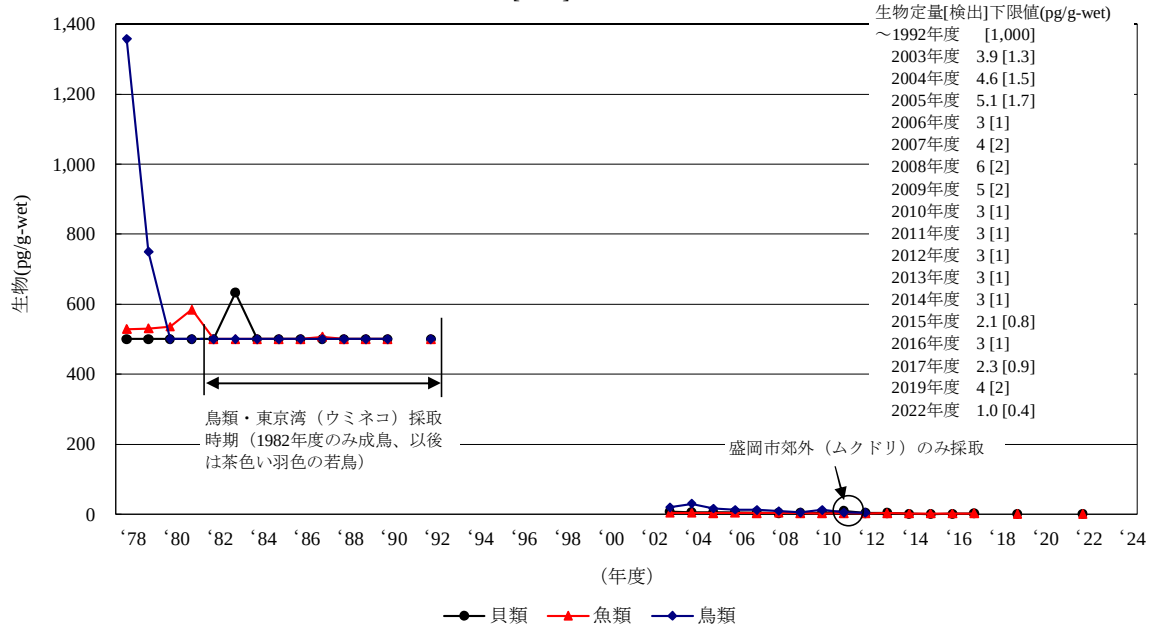
[11-4] \delta -HCH
