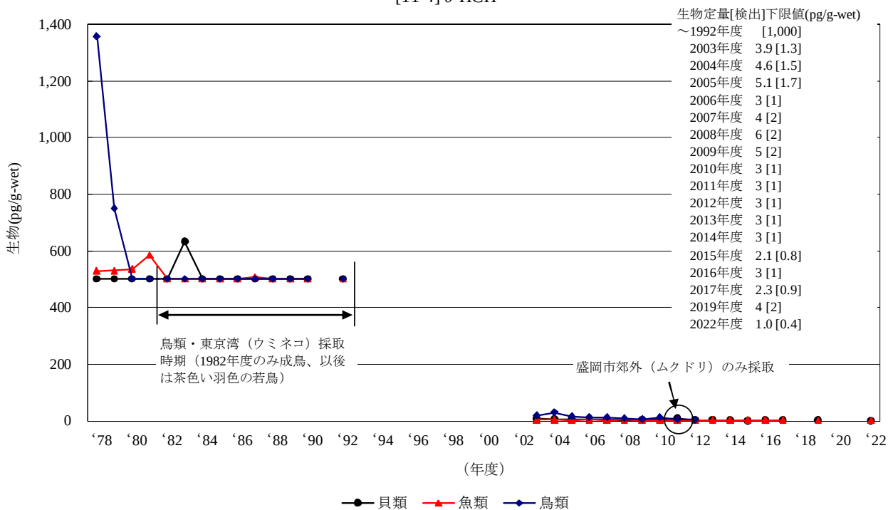
[11-4] \delta -HCH
