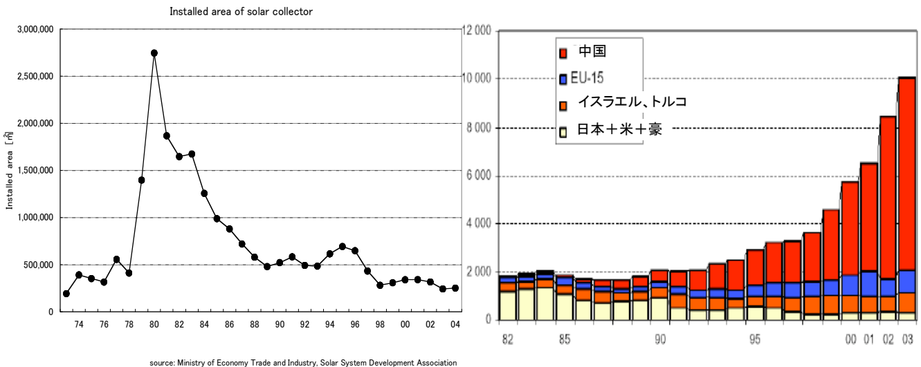
Solar heat (Glazed collectors) [MW/a] Sources: IEA SHC, ESTIF
