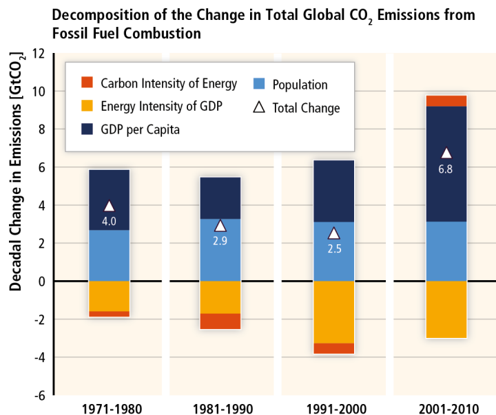
Figure SPM.3. Decomposition of the decadal change in total global CO 2 emissions from fossil fuel combustion by four driving factors; population, income (GDP) per capita, energy intensity of GDP and carbon intensity of energy. The bar segments show the changes associated with each factor alone, holding the respective other factors constant. Total decadal changes are indicated by a triangle. Changes are measured in giga tonnes (Gt) of CO 2 emissions per decade; income is converted into common units using purchasing power parities. [Figure 1.7] [Subject to final quality check and copy edit.]
