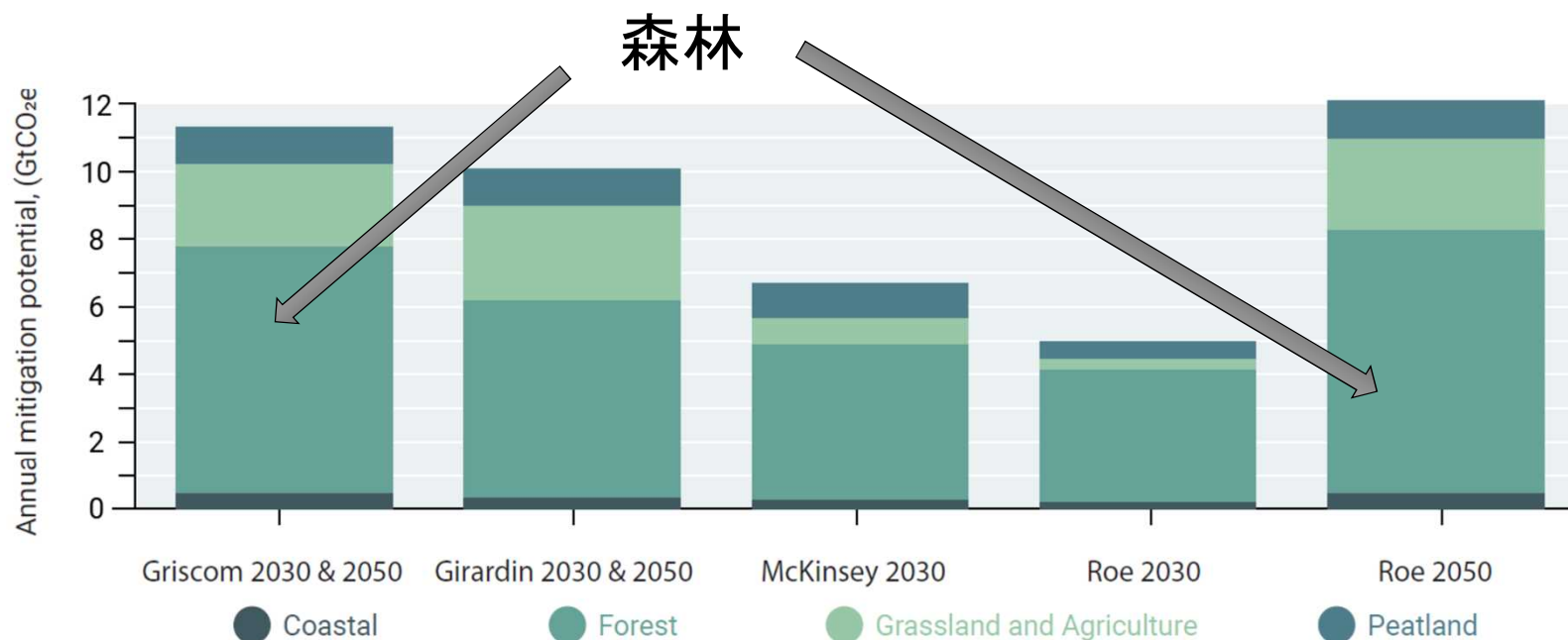
Figure 3: Global mitigation potential is spread across ecosystems, with all studies concluding that actions in forest have the greatest total potential
