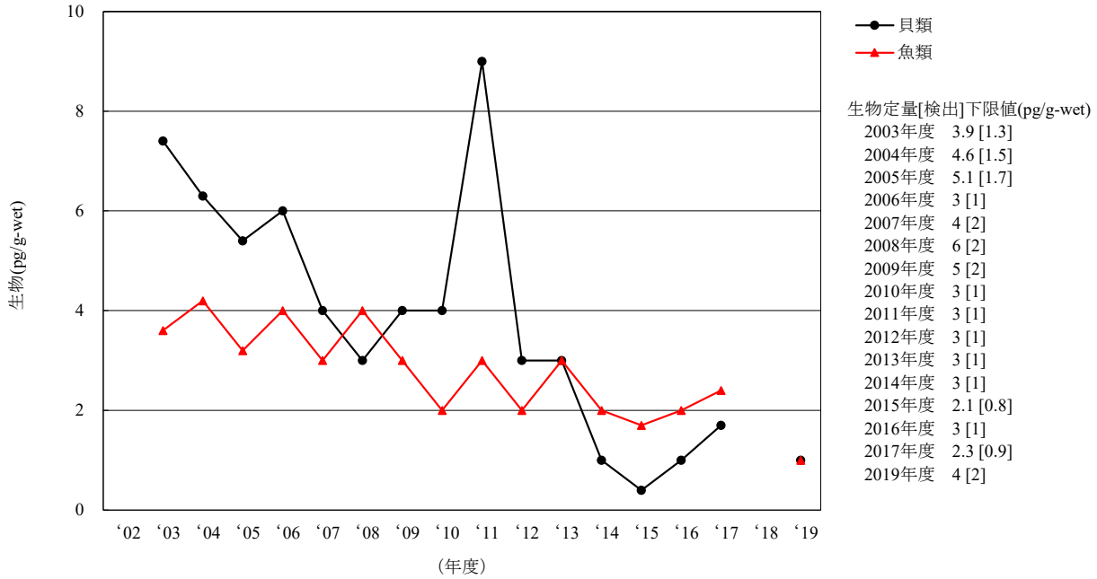
[11-4] δ-HCH
