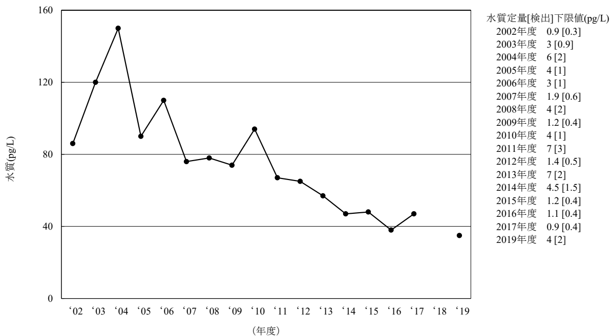
[11-1] \alpha -HCH
