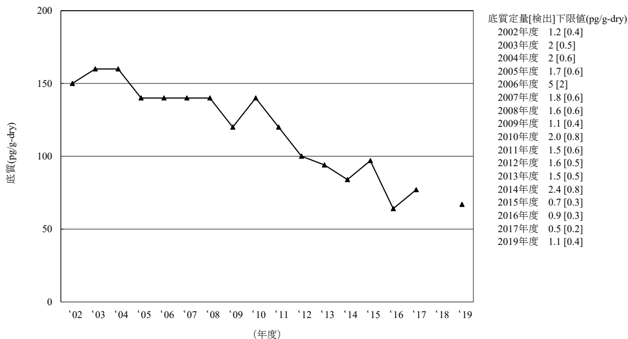
[11-1] \alpha -HCH
