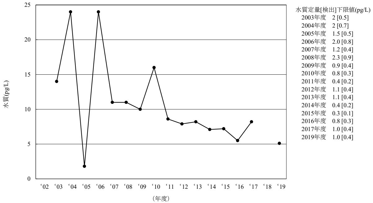
[11-4] \delta -HCH
