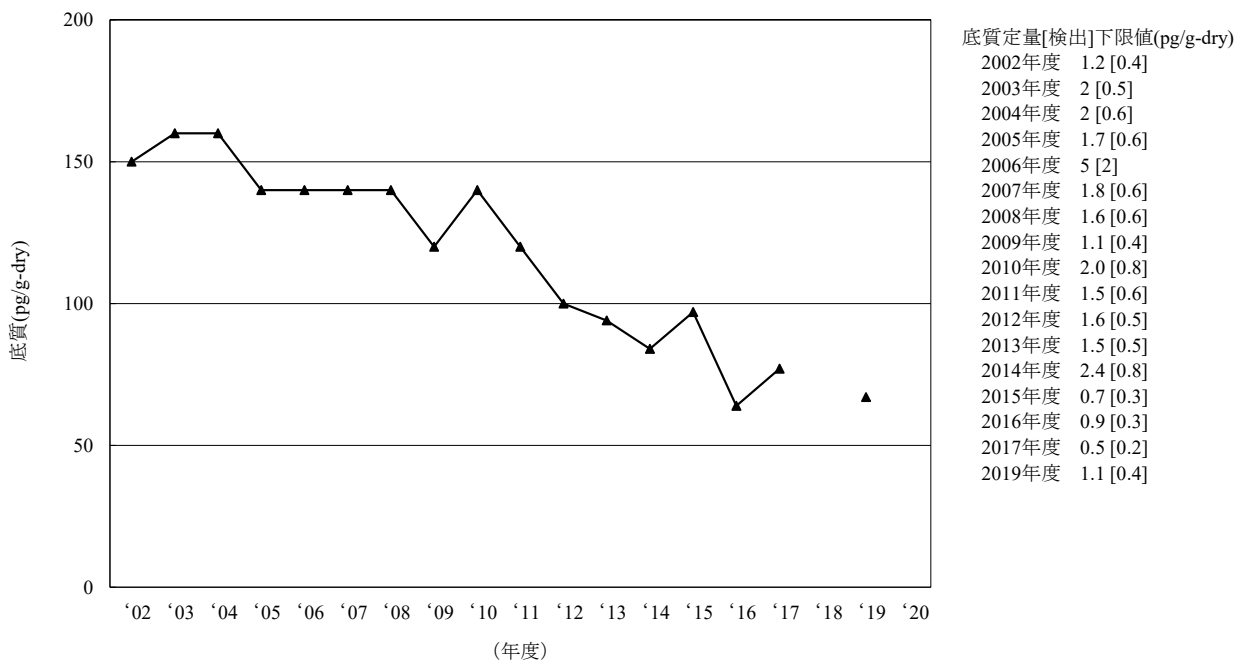
[11-1] \alpha -HCH
