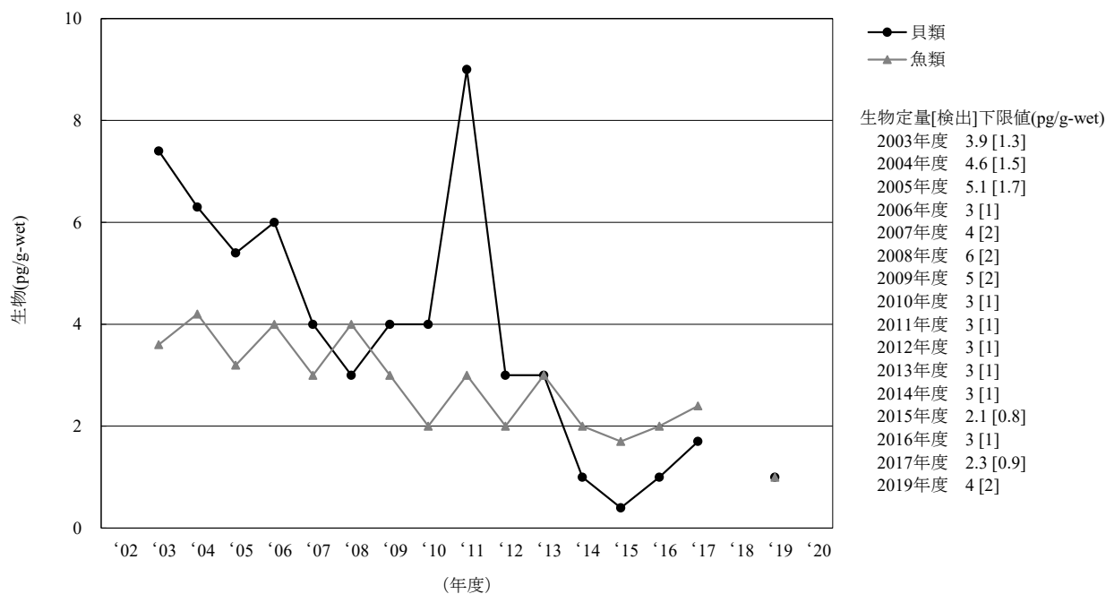
[11-4] δ-HCH
