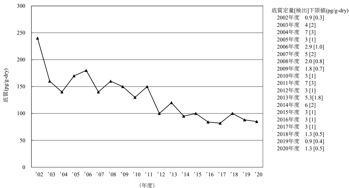
[2] HCB
