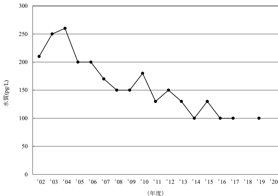
[11-2] \beta -HCH
