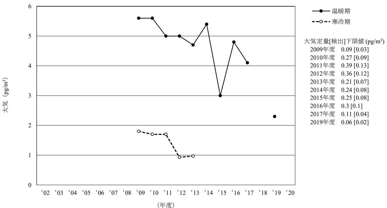
[11-2] \beta -HCH
