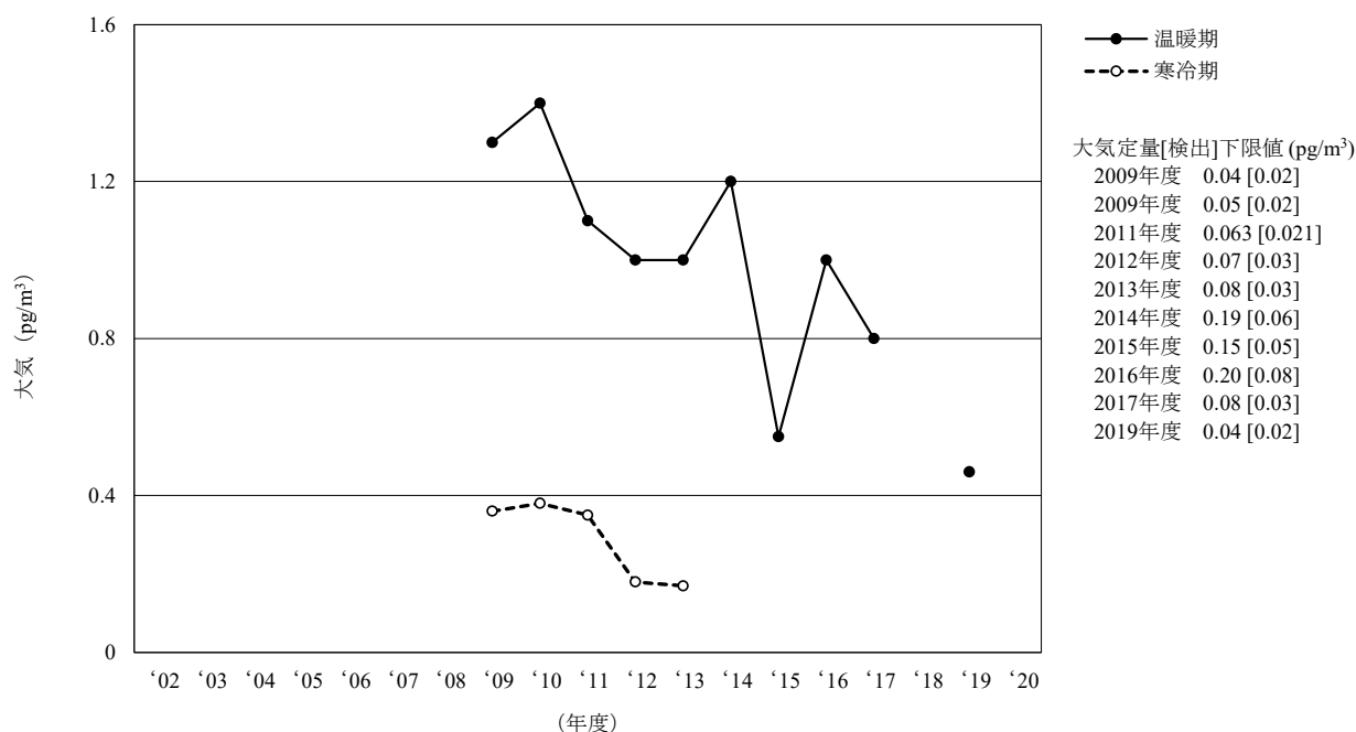
[11-4] δ-HCH
