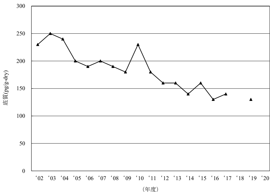
[11-2] \beta -HCH
