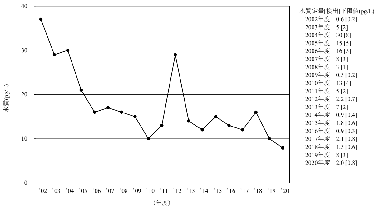
[2] HCB
