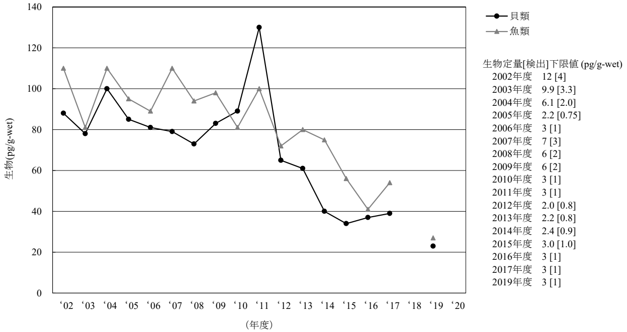
[11-2] \beta -HCH
