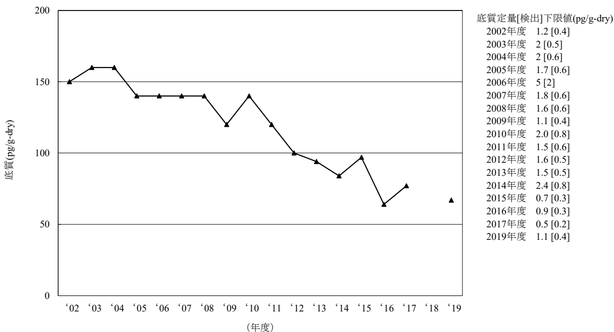
[11-1] \alpha -HCH
