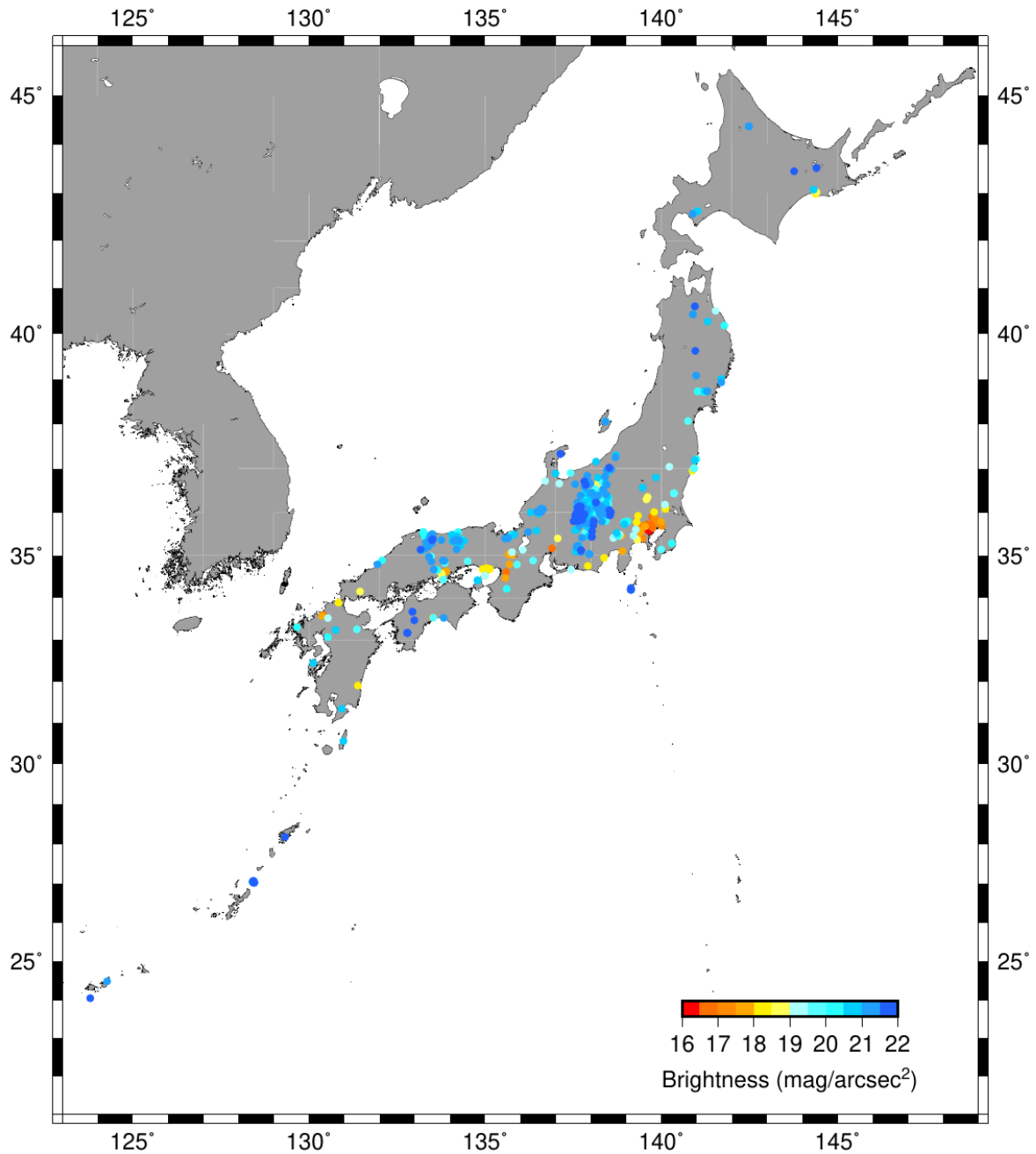
Night Sky Brightness of Japan (10 – 23 Aug, 2020)
