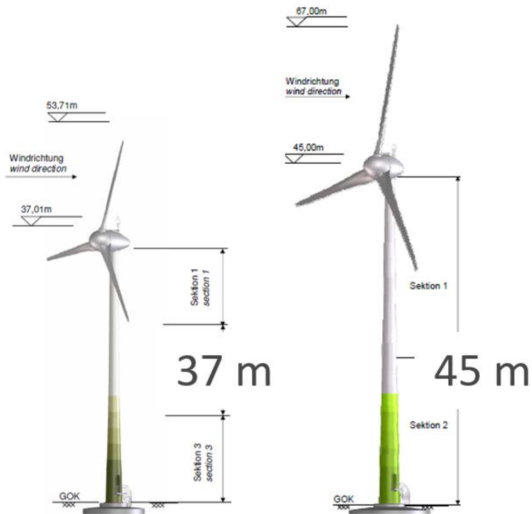
Figure 52: Relative size of the current E33 wind turbines (left) and the proposed E44 wind turbines (right).
