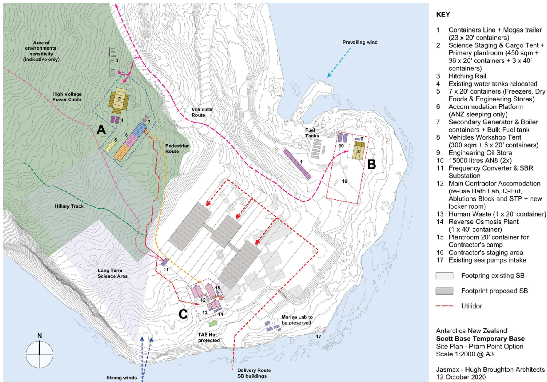
Figure 38: Site plan indicating the current, proposed station and temporary base location.
