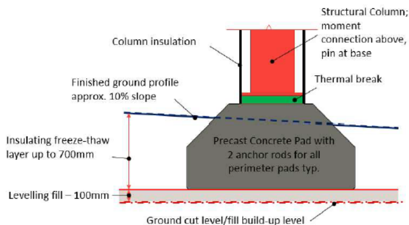
Figure 63: Diagram illustrating the proposed pad foundation option.
