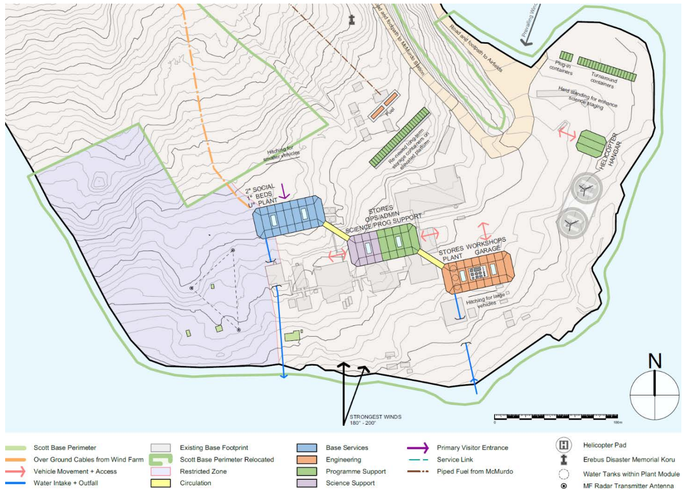
Figure 60: Concept Design D - plan view.
