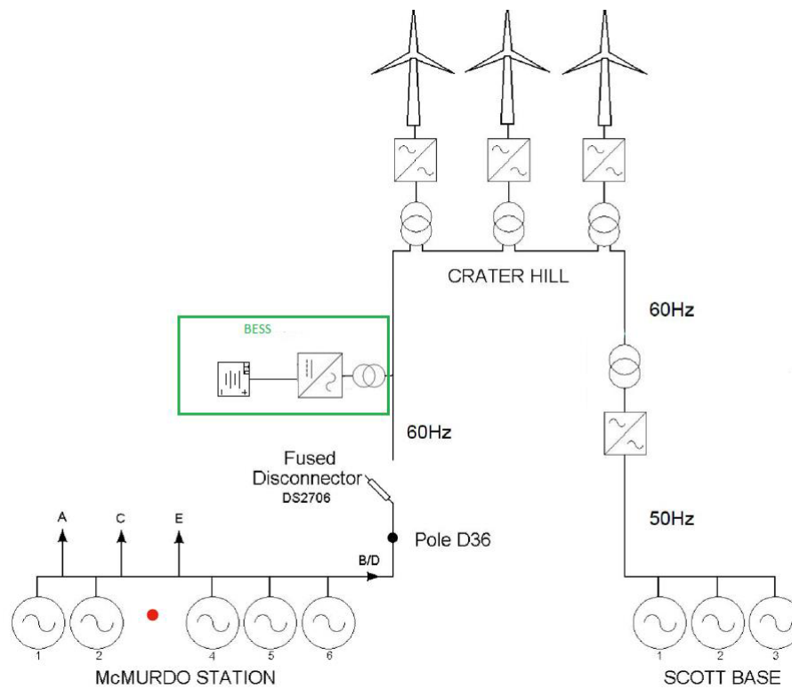
Figure 50: Power system concept design indicating from left to right, the McMurdo generators and distribution, the proposed BESS, proposed turbines, frequency converter, and Scott Base generators.
