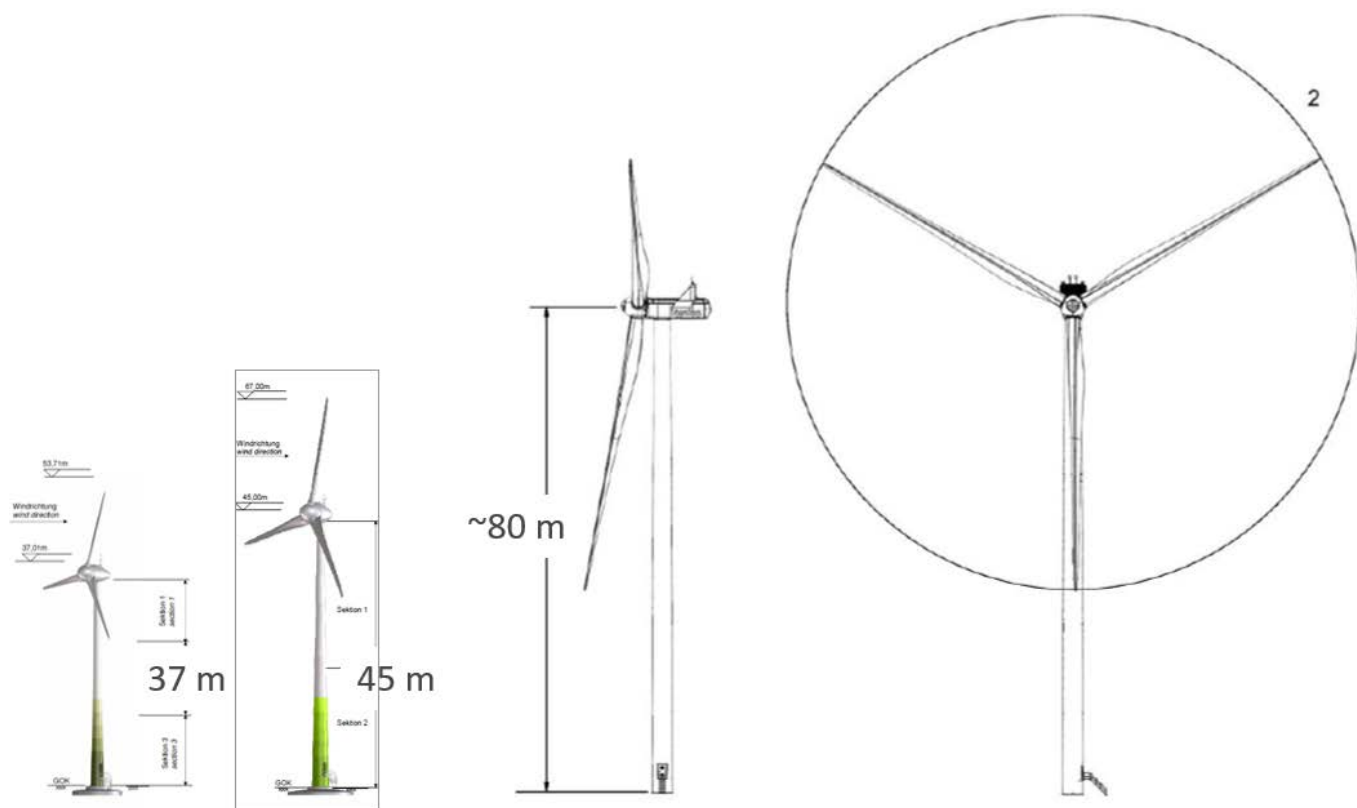
Figure 67: Relative size of wind turbines. From left, current E33, E44, E115.
