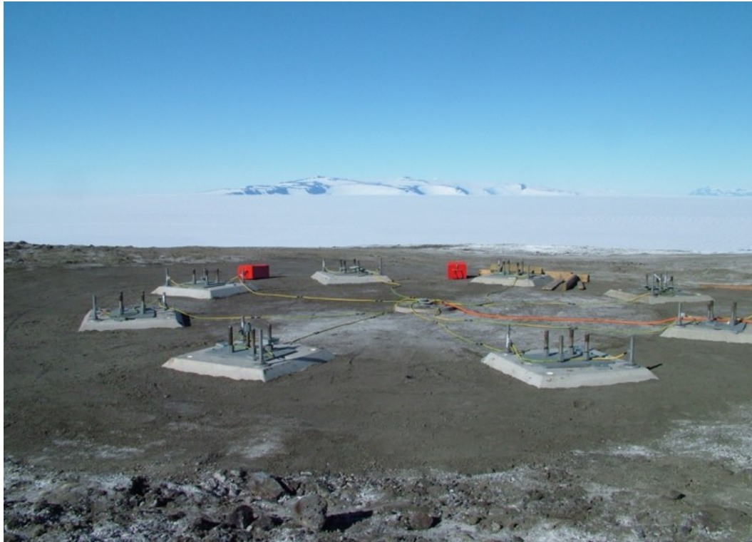
Figure 53: Pre-cast concrete foundation footings backfilled so only the top is visible.
