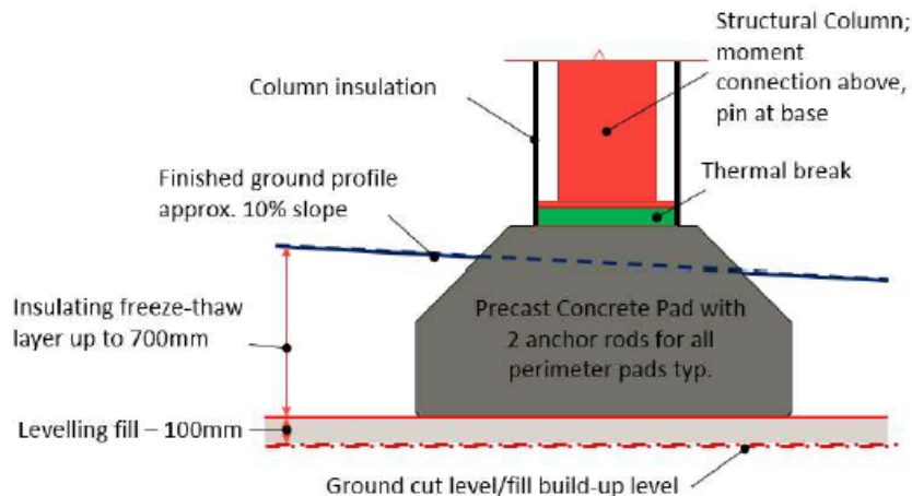
Figure 42: Pad foundations proposed for the temporary base buildings.
