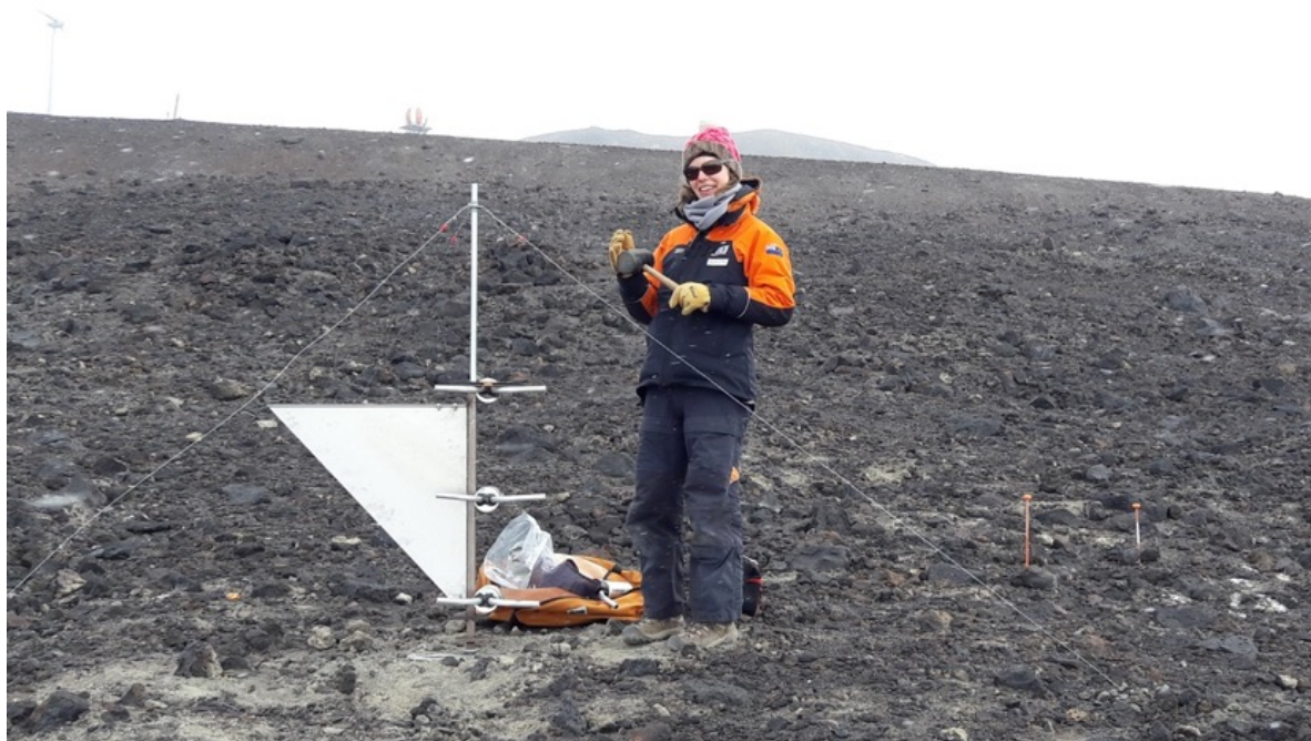
Figure 107: An MWAC dust sampler being installed at one of the monitoring sites behind the current Scott Base. Photo: O'Neill, University of Waikato.
