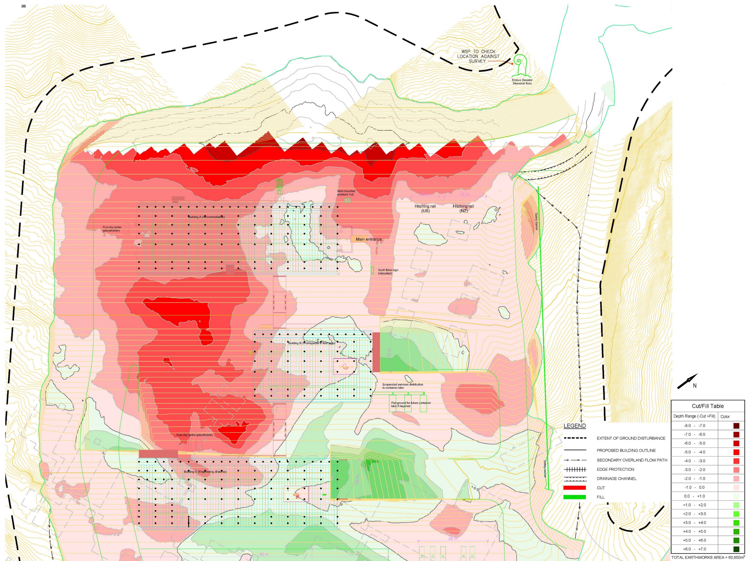
Figure 29: Detail of bulk earthworks plan with pile locations for the proposed Scott Base buildings (WSP, 2020).
