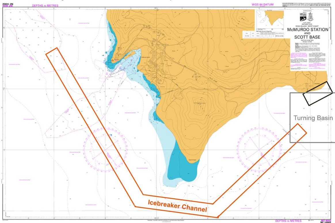
Figure 48: Indicative location of the additional icebreaker channel required to reach Pram Point.
