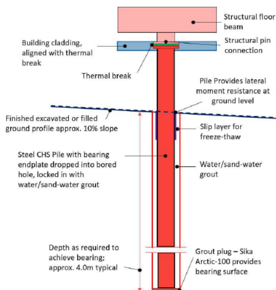
Figure 33: Sketch of the proposed end-bearing pile.
