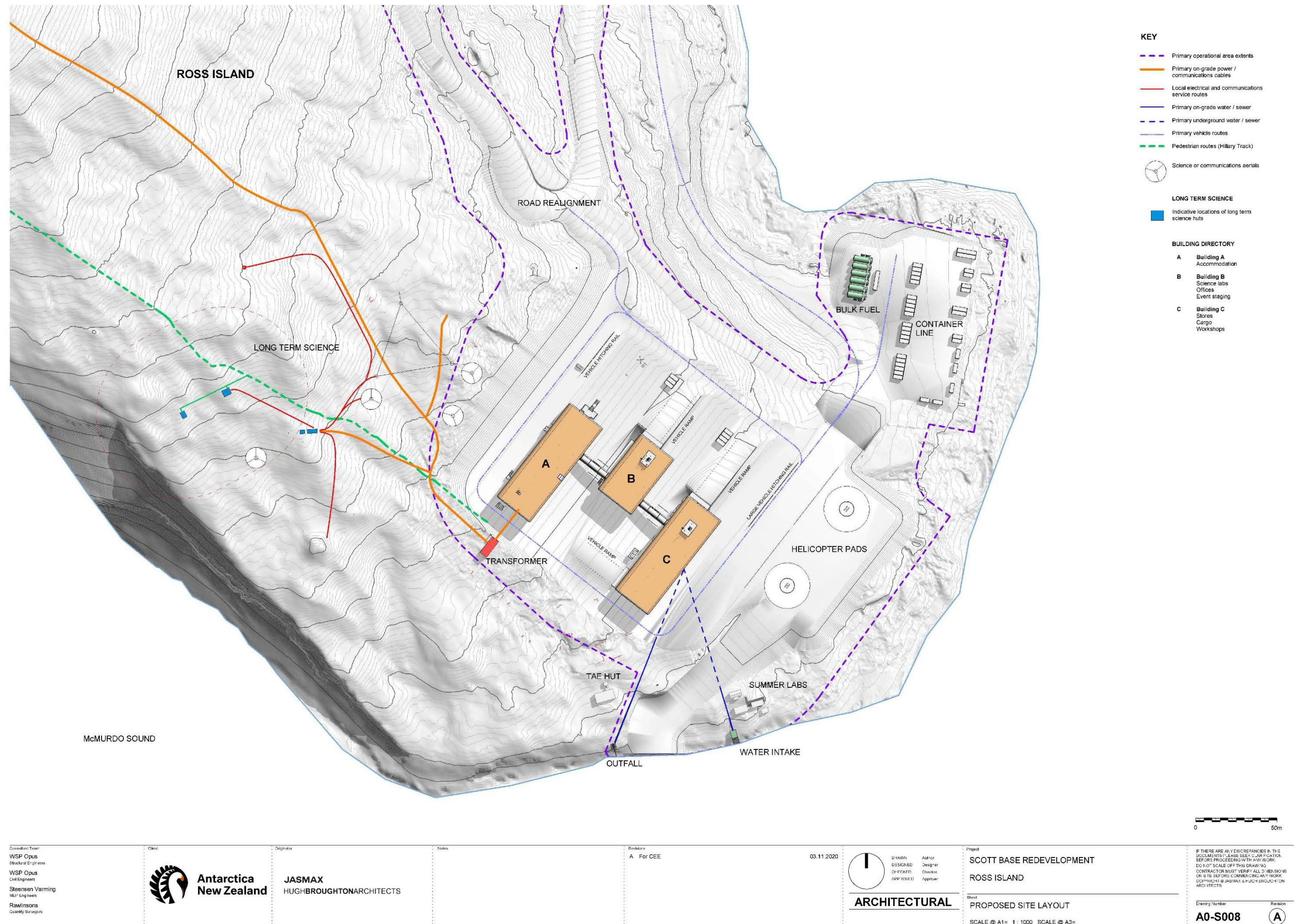
Figure 22: Proposed site layout at Pram Point.
