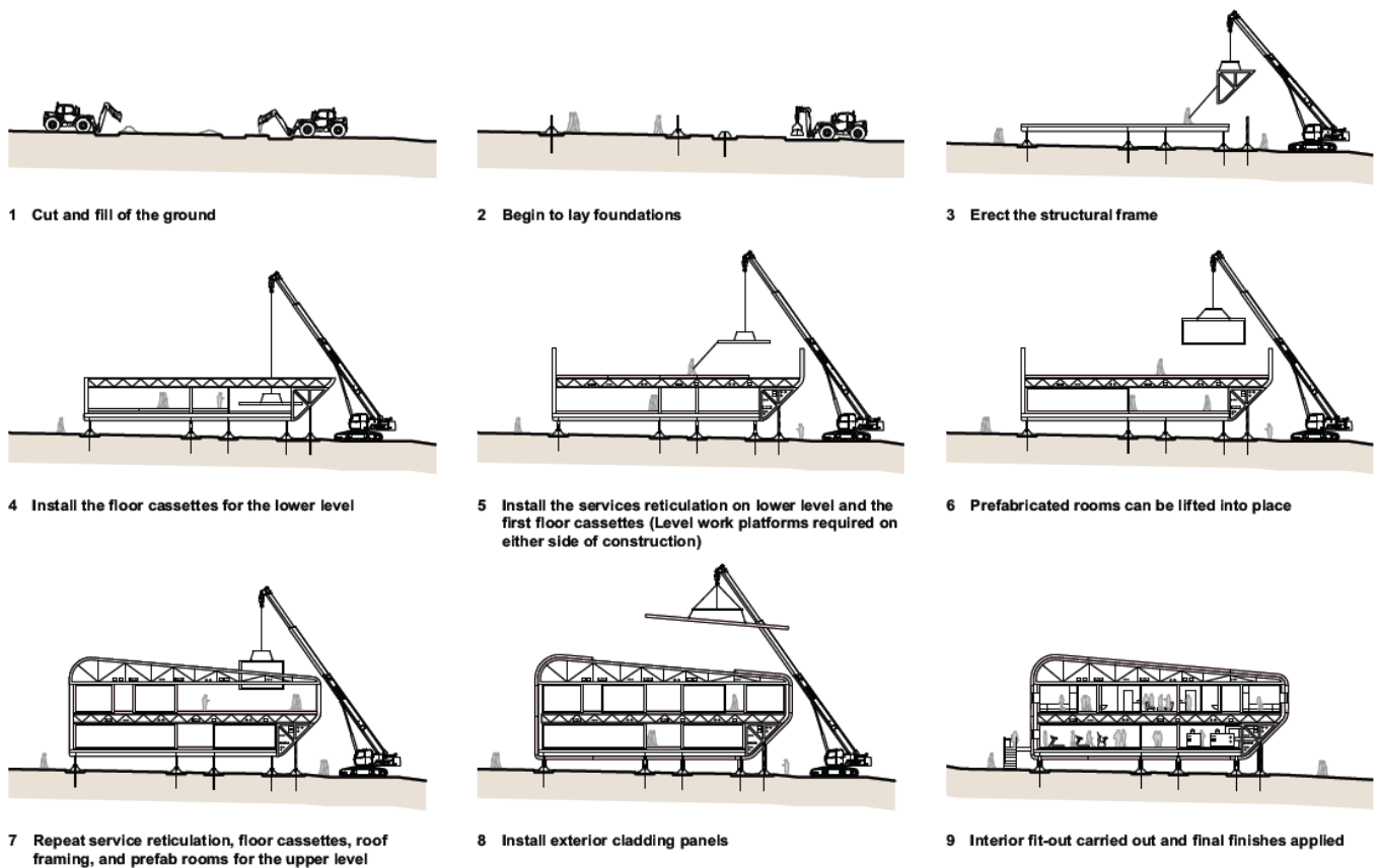
Figure 65: Construction sequencing for a traditional build on site.
