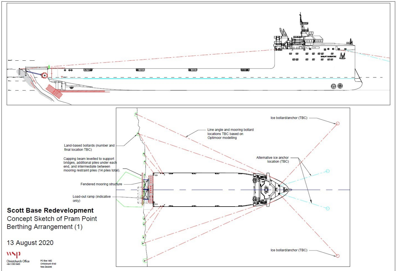
Figure 45: Plan and elevation view of the berthing arrangement.
