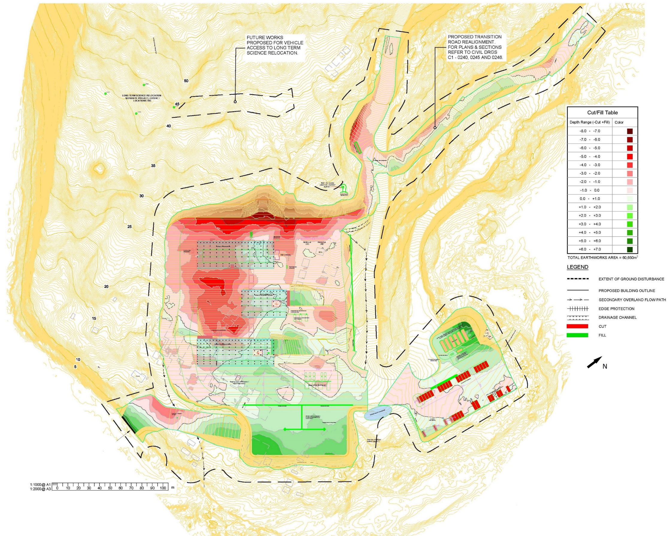
Figure 28: Bulk earthworks plan for the Scott Base Redevelopment with proposed locations of the three buildings, all associated infrastructure and relative locations of the current facilities (WSP, 2020).
