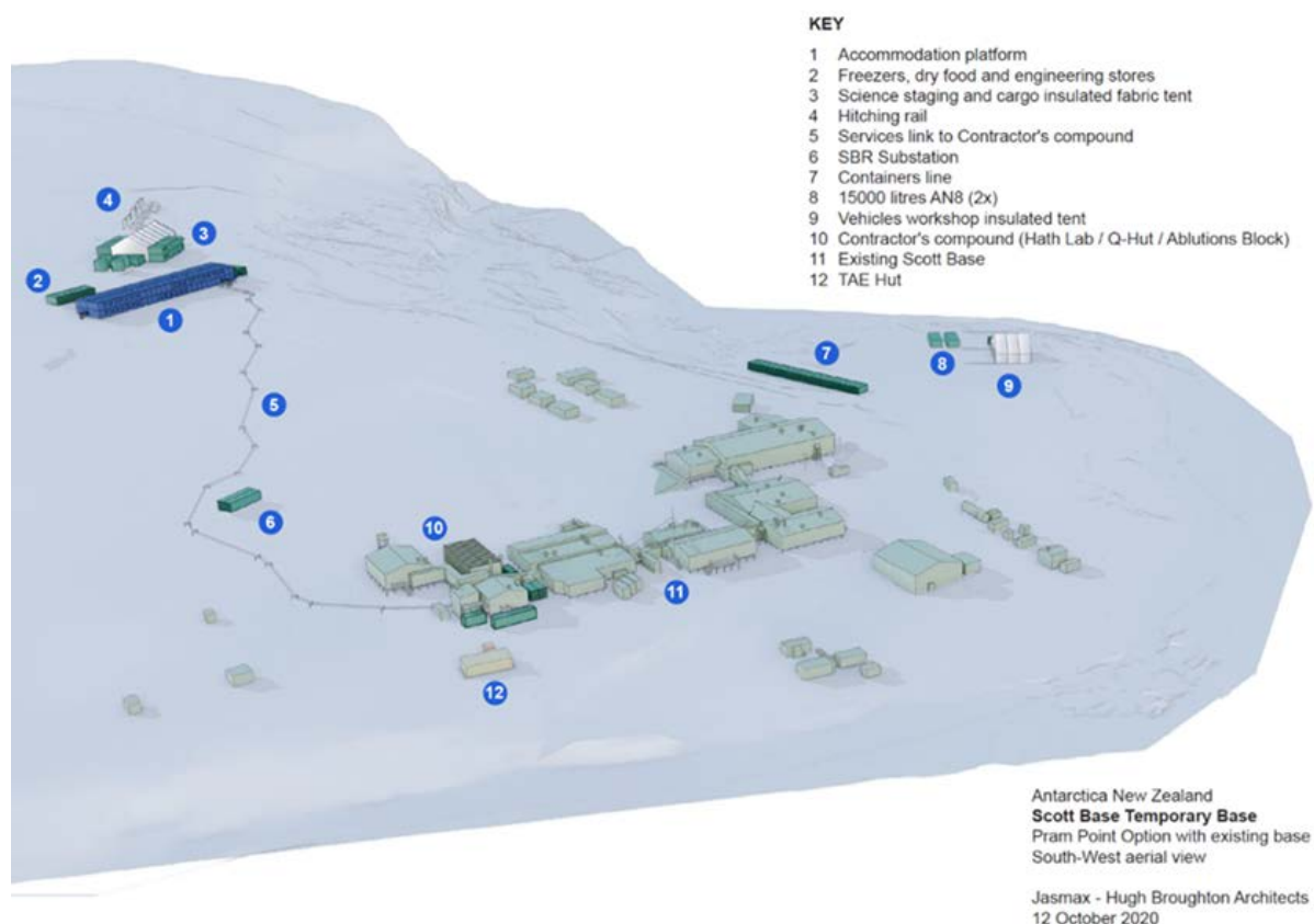
Figure 39: Temporary base design and location in relation to the current Scott Base.
