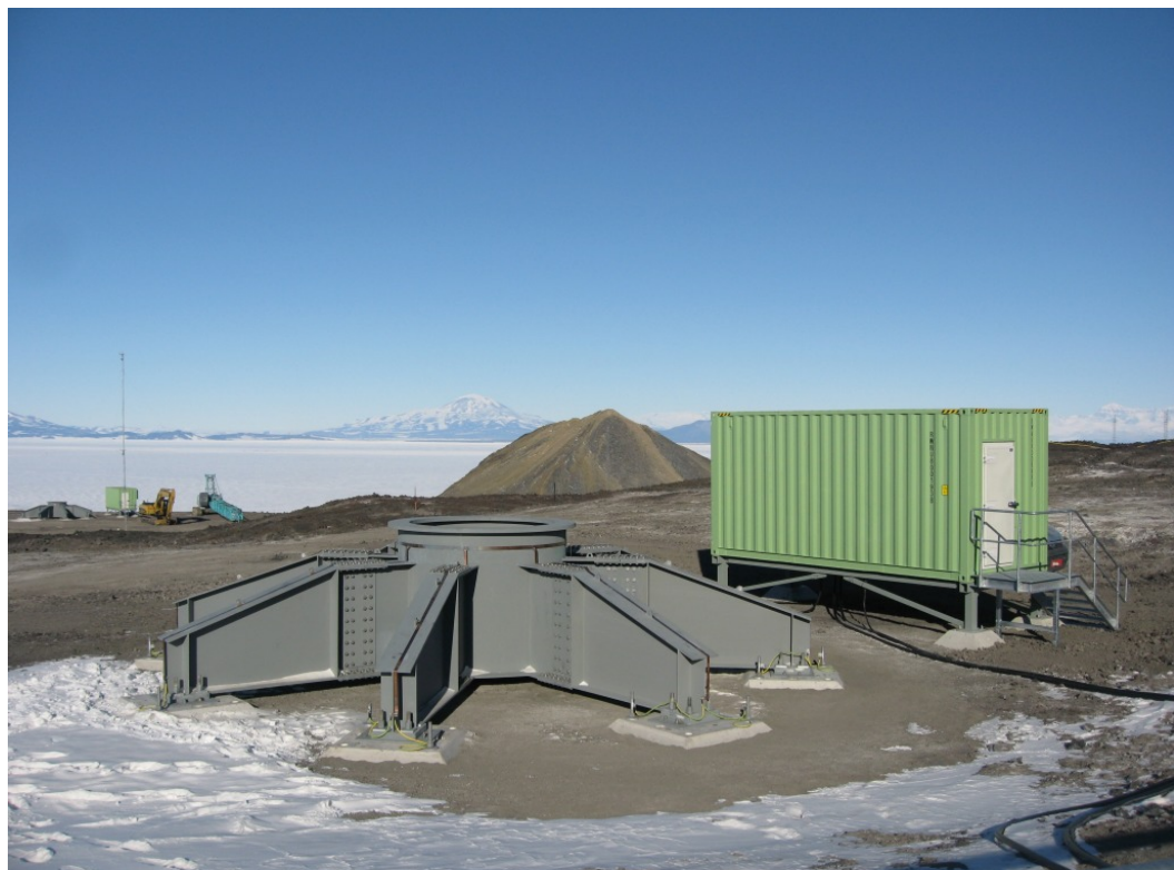
Figure 54: Steel spider framework bolted to the concrete foundation blocks.
