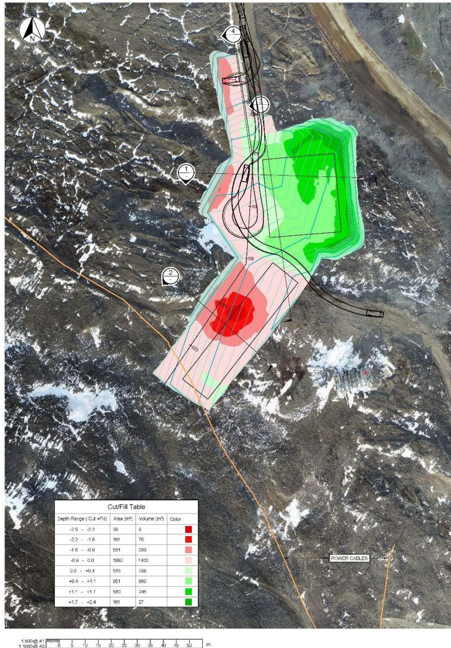
Figure 41: Preliminary temporary Scott Base Area A earthworks requirements.
