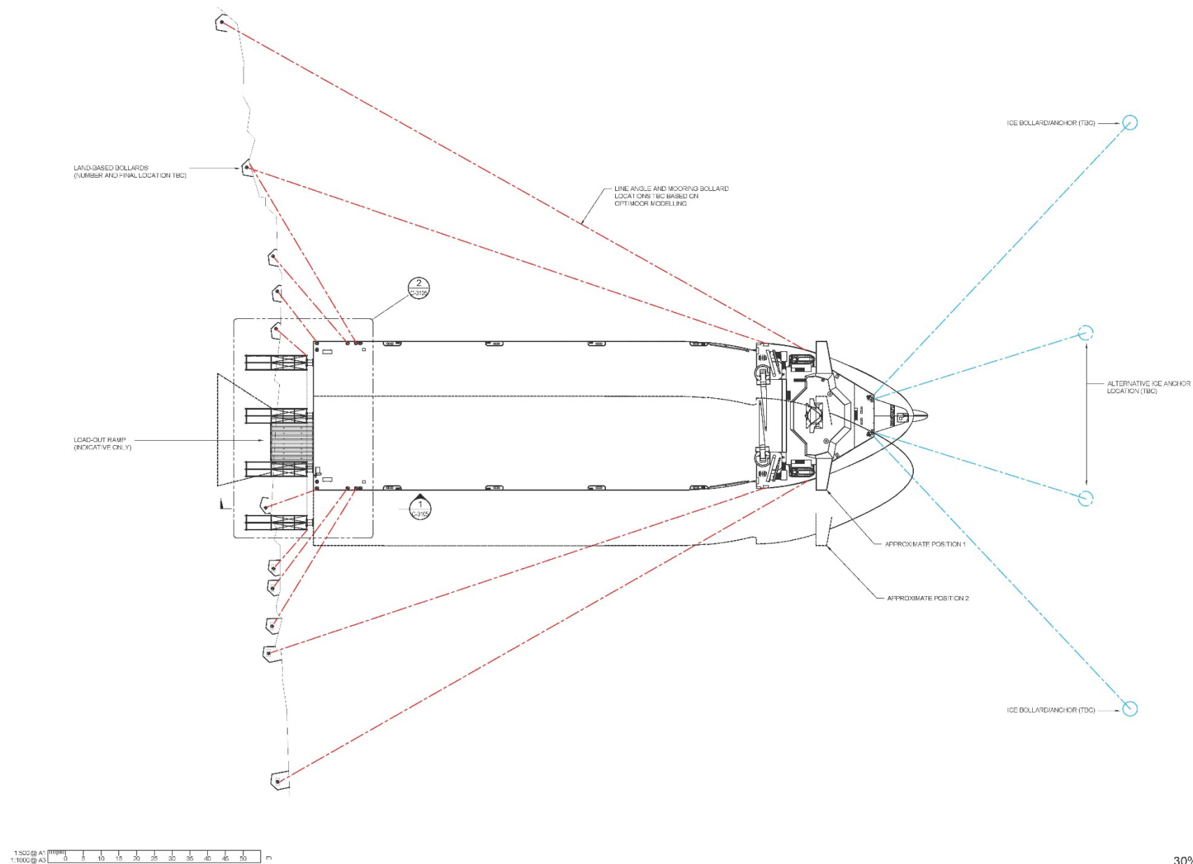
Figure 37: Detail of the mooring location and two ship docking positions. Mooring lines and bollards are detailed.
