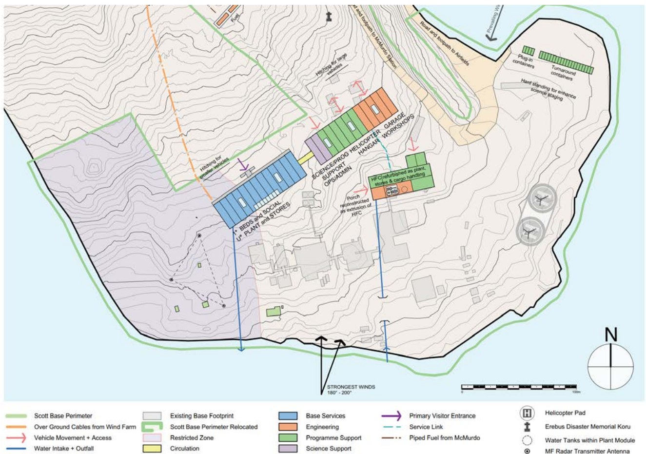
Figure 58: Concept Design B - plan view.
