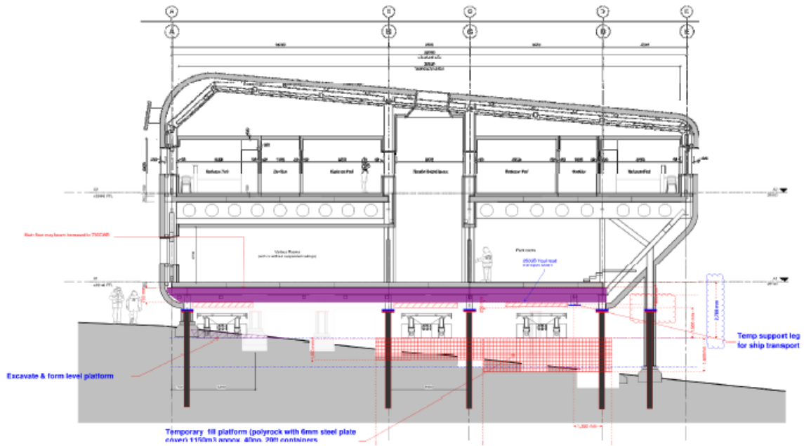
Figure 47: Side view of SPMTs delivering a building module to site. Red hash denotes the temporary platform due to gradient differences across the building platform.
