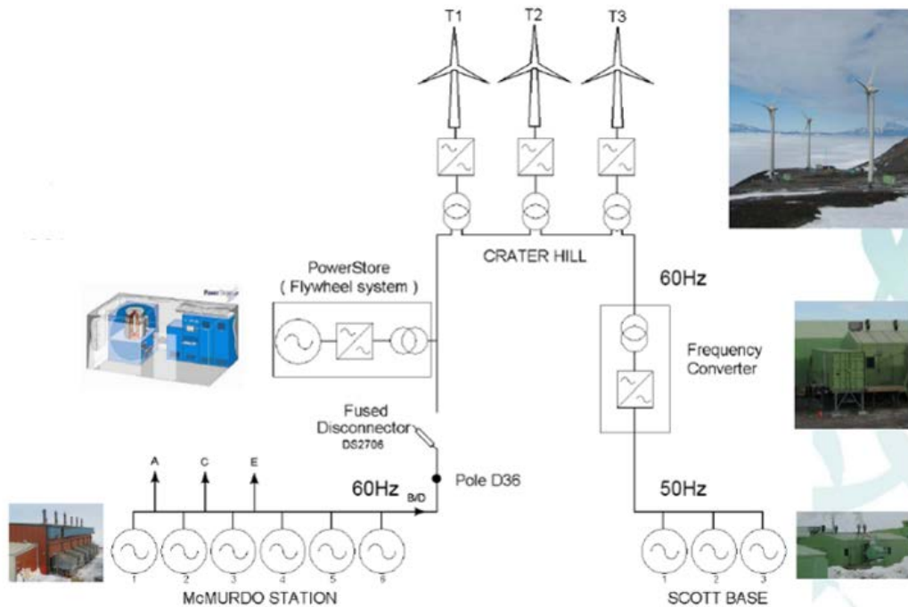
Figure 49: Current RIWE system design.
