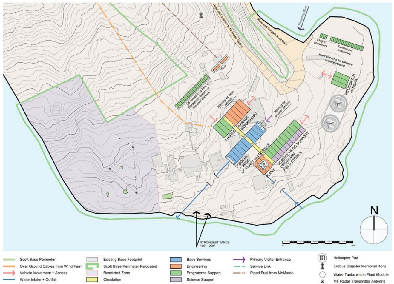
Figure 59: Concept Design C - plan view.
