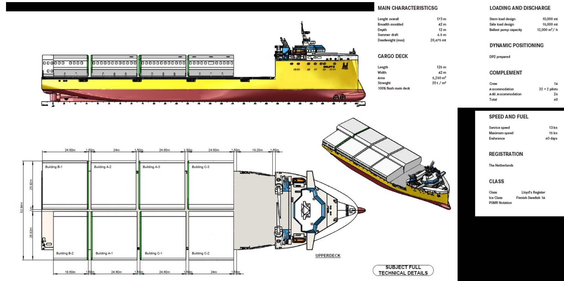
Figure 43: Preliminary loading arrangement and characteristics of the proposed MC Class vessel for the delivery of the building modules 17 .
