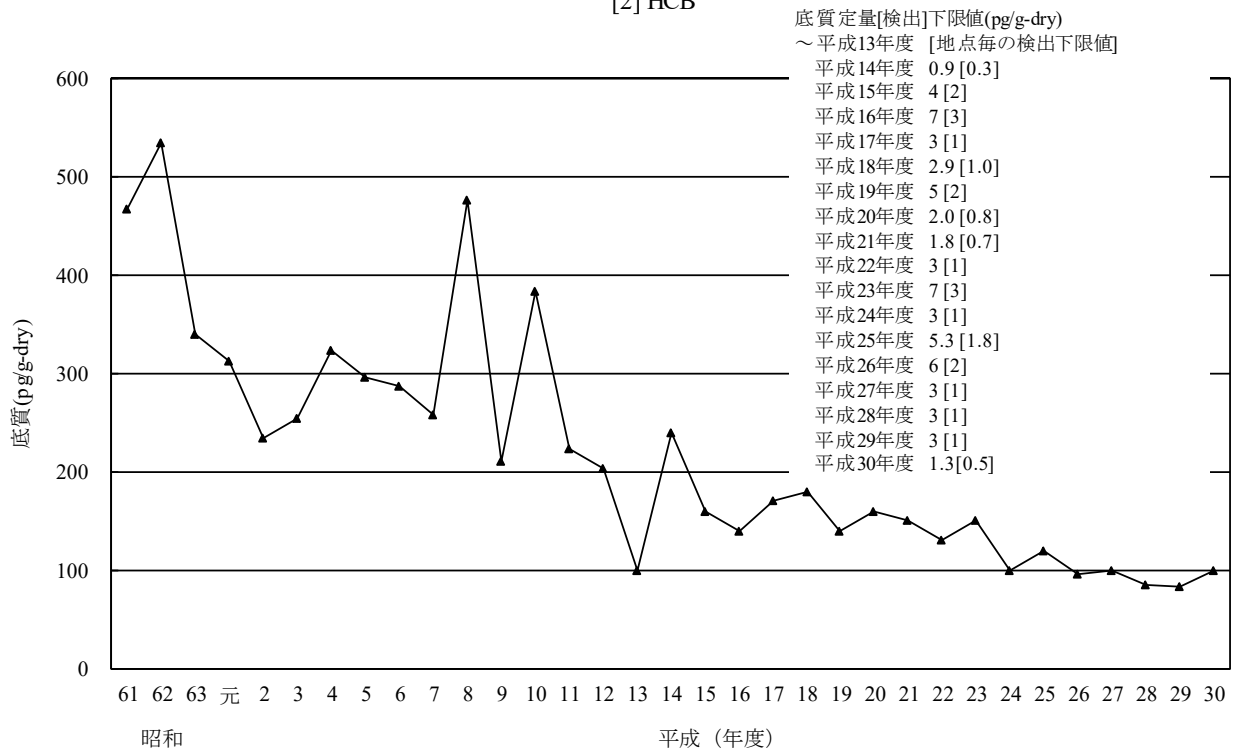
[2] HCB
