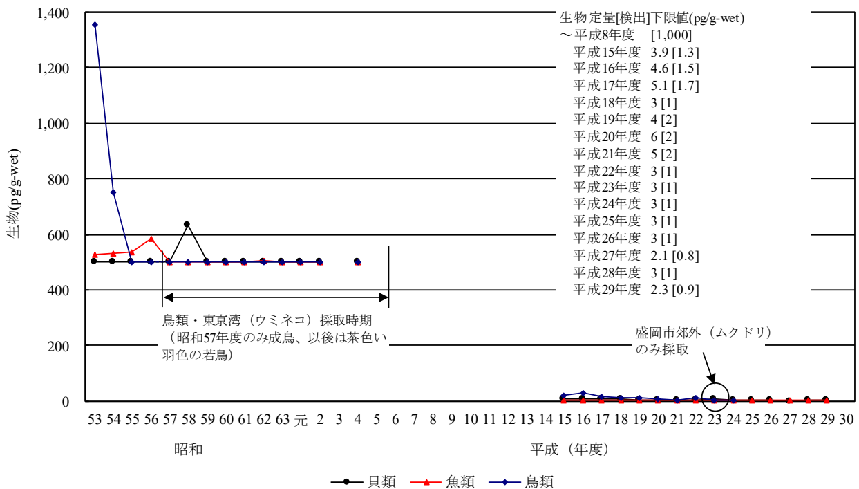
[11-4] \delta -HCH
