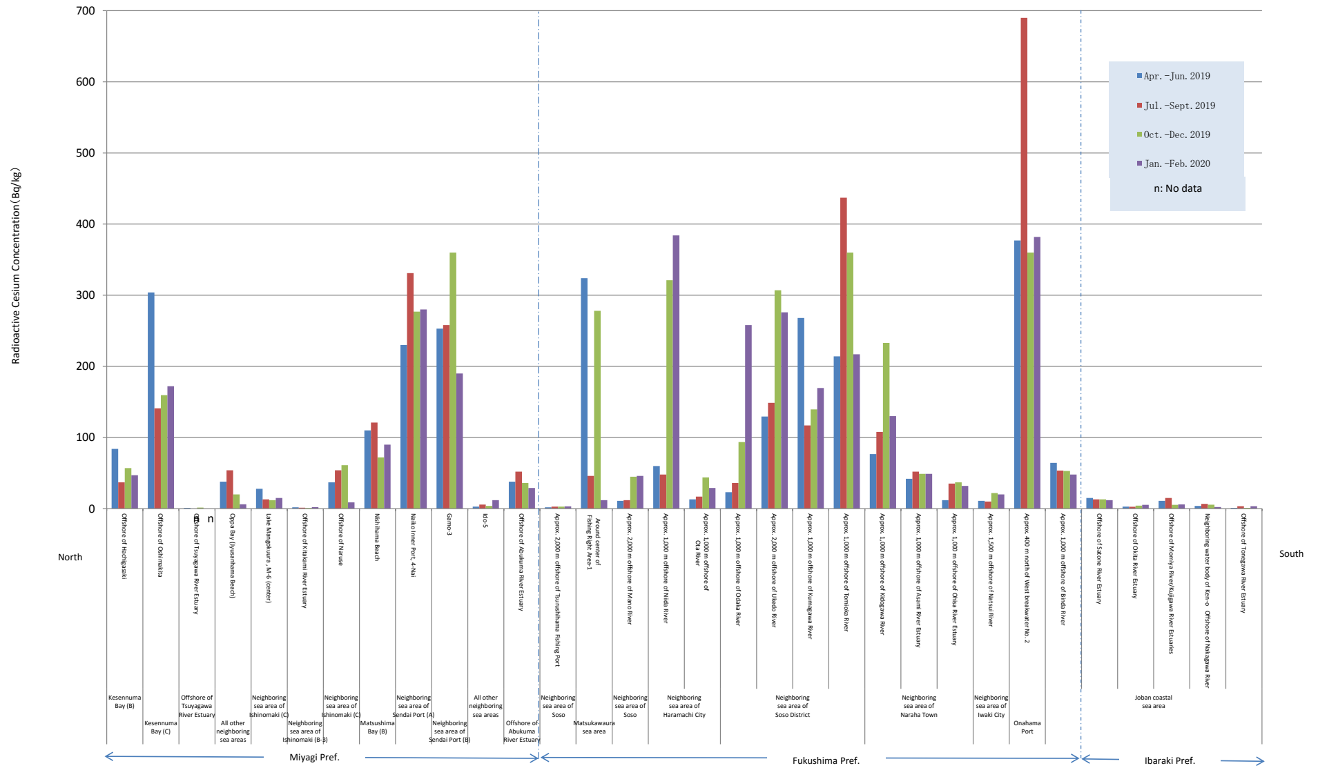
Sea areas from the coast(Sediment):Changes in radioactive cesium concentration (Miyagi,Fukushima,and Ibaraki Prefectures)(FY2019)
