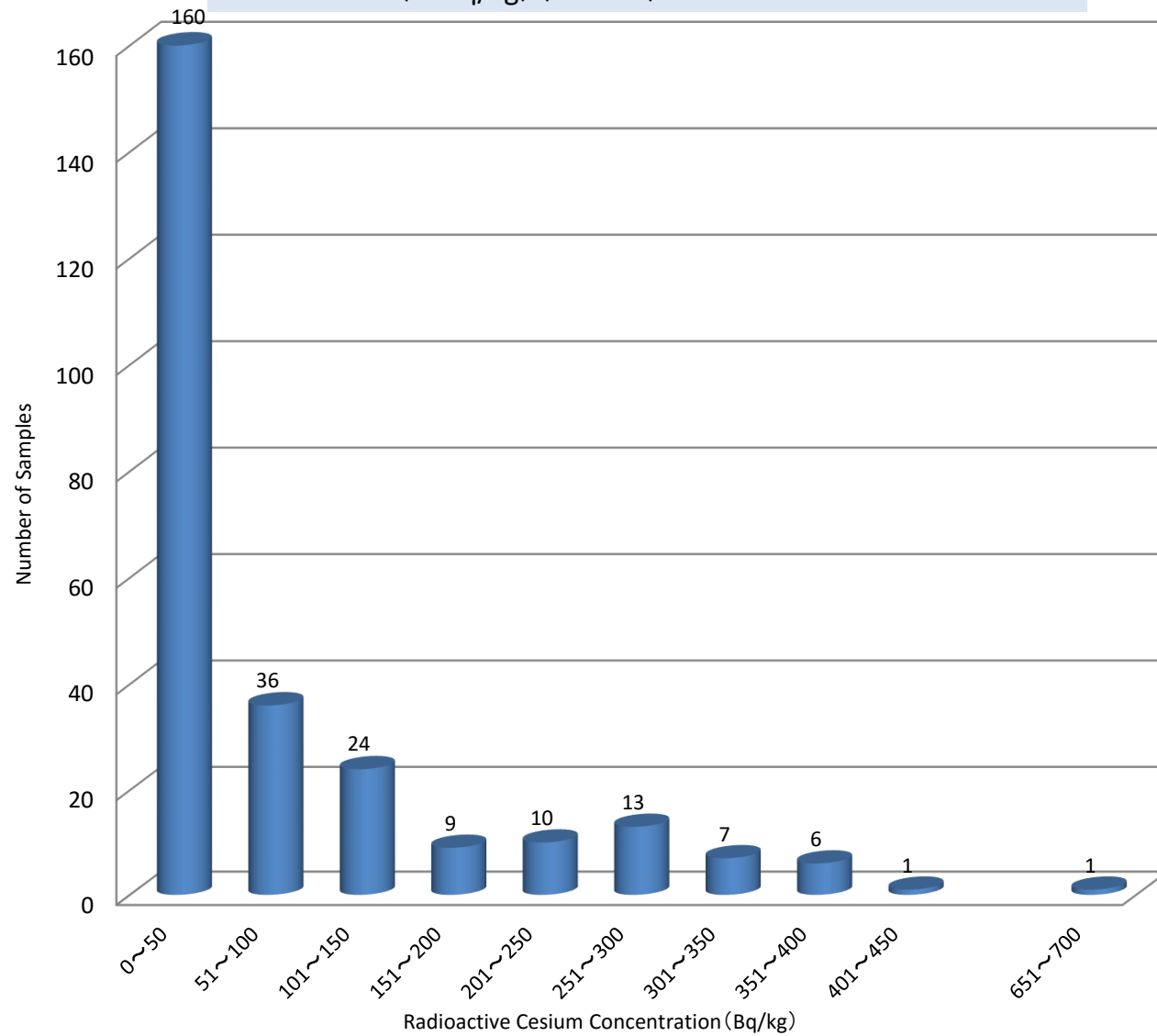
Coastal areas(Sediment):Number of Samples by radioactive cesium concentration (50Bq/kg) (FY2019)
