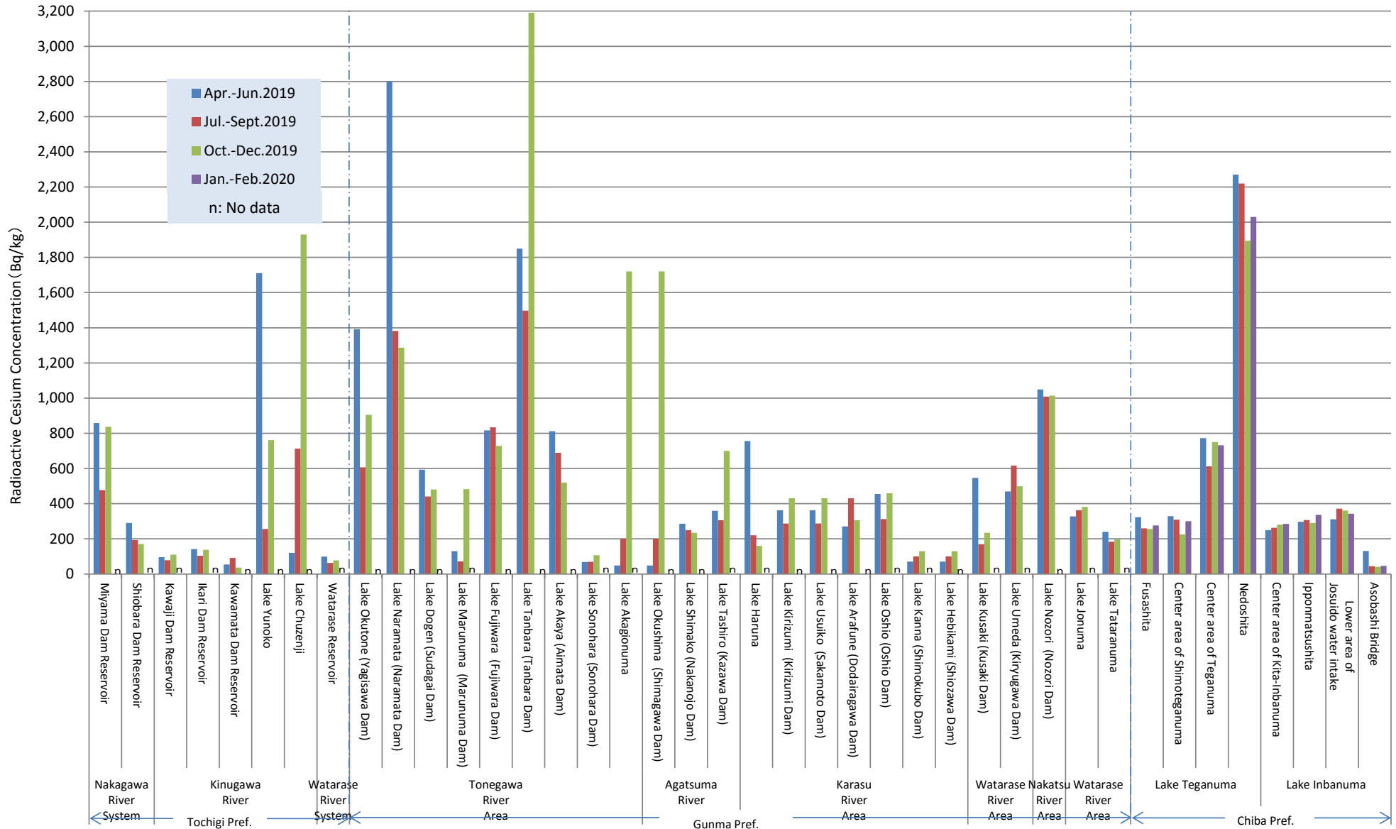
Lakes(Sediment):Changes in radioactive cesium concentration (Tochigi, Gunma, and Chiba Prefectures)(FY2019)
