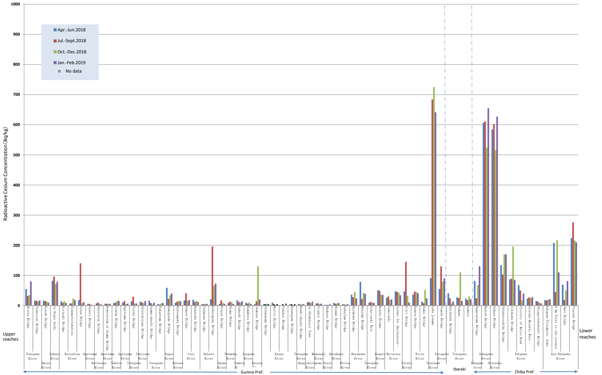
Rivers (Sediment):Changes in radioactive cesium concentration (Tone River System)(FY2018)
