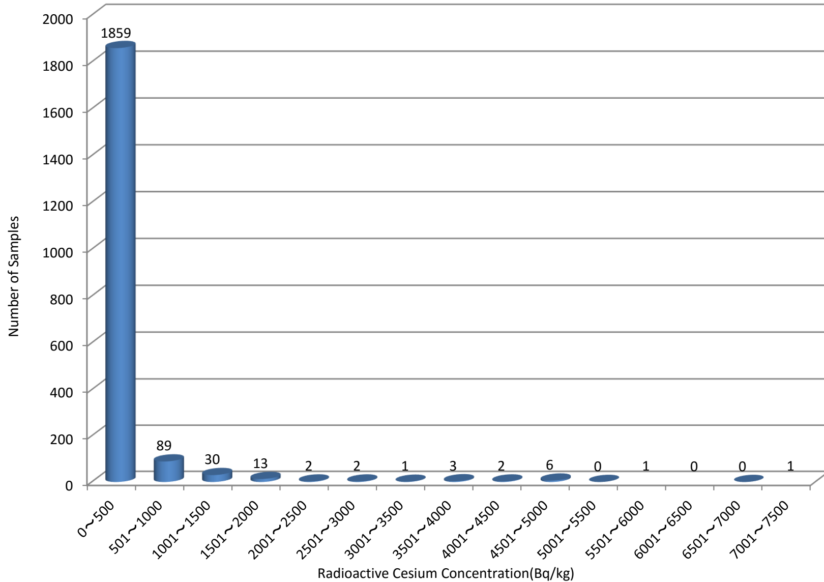
Rivers(Sediment):Number of Samples by radioactive cesium concentration (500Bq/kg) (FY2018)
