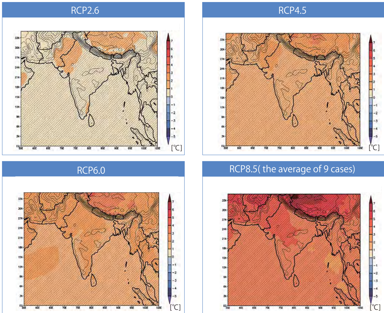
Fig. 1 Changes in annual mean surface temperatures ( ^{\circ}\text{C} ) in South Asia under each RCP scenario. Differences in temperatures between present climate (1984-2004) and future climate (2080-2100) are shown. Colors indicate average values of the three cases under the RCP2.6, 4.5, and 6.0 scenarios, as well as those of the nine cases under the RCP8.5 scenario, and the meshing indicates the areas where the tendency of future changes agrees among all cases (areas with high confidence). For reference, the topography of the climate model is shown with contour lines (the topography is modeled; therefore, it may differ from the actual topography).
