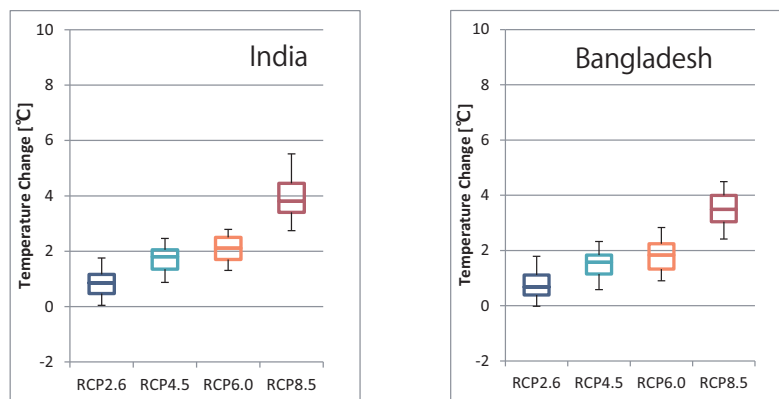
Fig. 2 Changes in annual mean surface temperatures ( ^{\circ}\text{C} ) under each RCP scenario in India (left) and Bangladesh (right). Summary of the magnitude of temperature increases for each RCP scenario. Box plots indicate 25-75 percentile ranges and central values, and error bars indicate 5-95 percentile ranges. The magnitude of temperature changes is indicated by the difference from the mean temperatures of the present climate (1984-2004). For each RCP scenario, aggregations are made for all years and for all cases.
