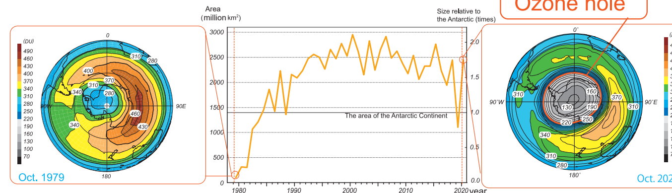
Changes in annual maximum of the ozone hole area (center) and the total ozone maps over the Antarctic region in October (left and right)
