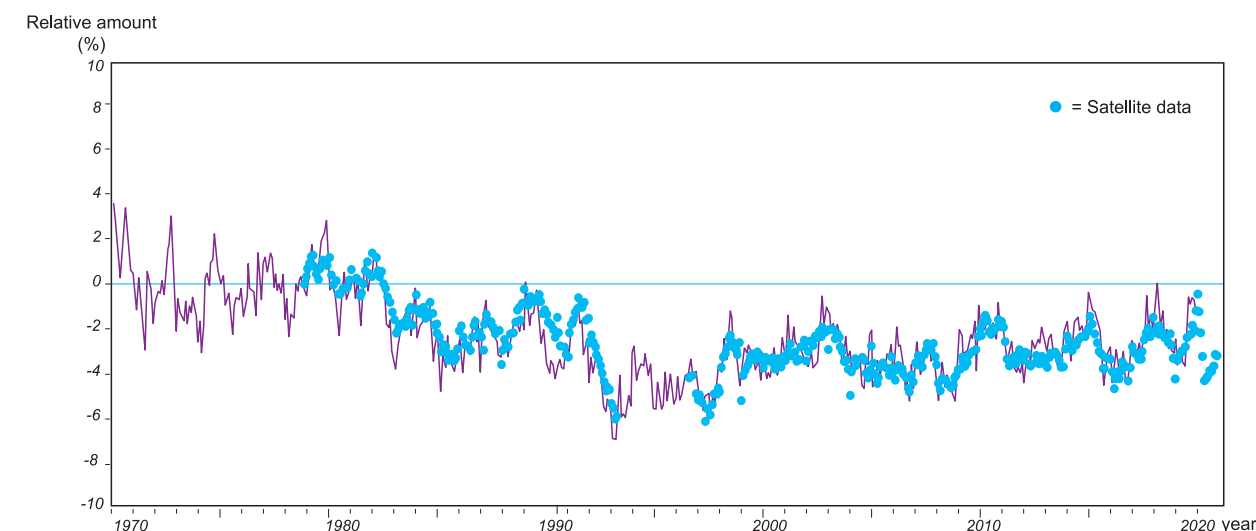
Time series in global mean total ozone
