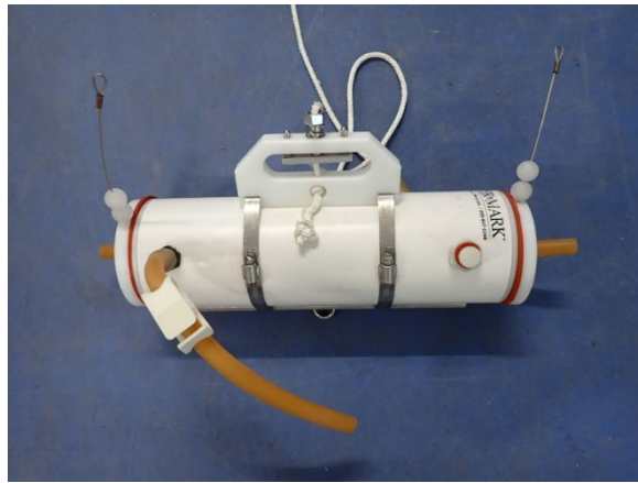
Figure 7. Van Dorn sampler
