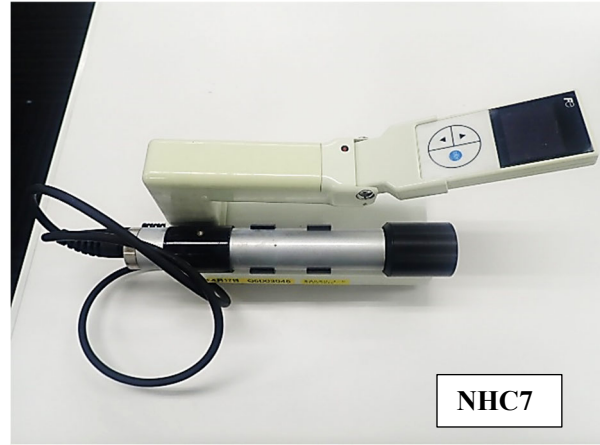
Figure 5. NaI (TI) scintillation survey meter
