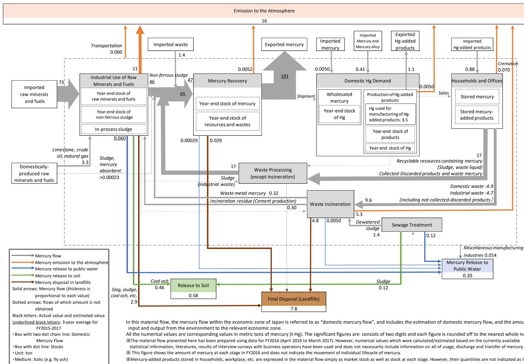
Mercury Material Flow in Japan (FY2016)
