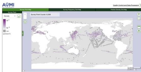
Survey point distribution and microplastic abundance map from AOMI website
