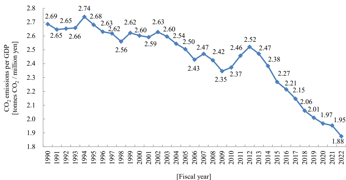
Figure 2-5 Trends in CO 2 emissions per unit of Real GDP
