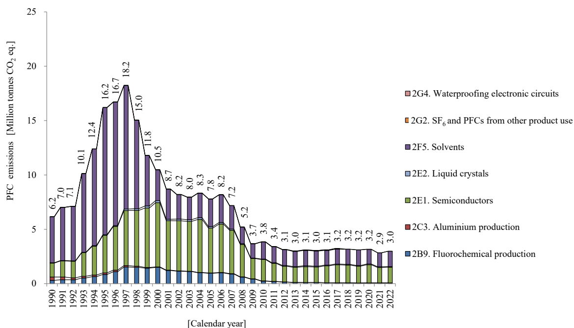
Figure 2-9 Trends in PFC emissions
