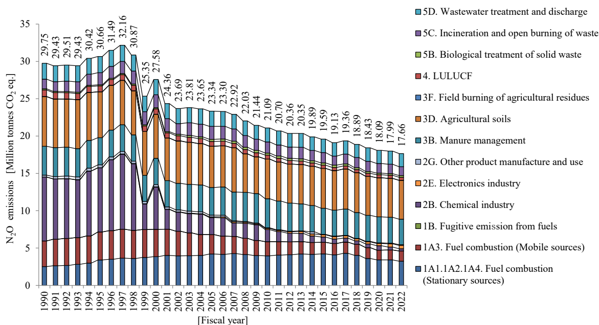
Figure 2-7 Trends in N 2 O emissions
