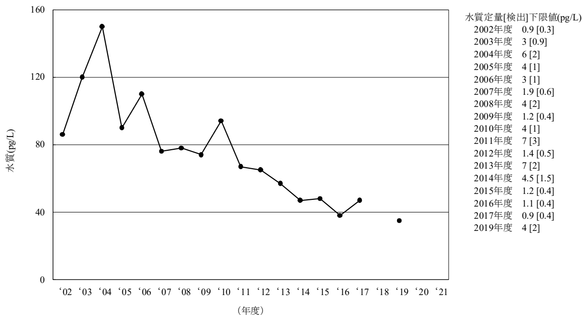
[11-1] \alpha -HCH
