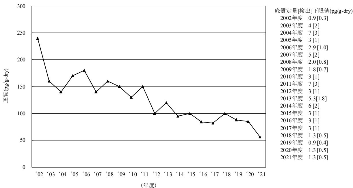
[2] HCB
