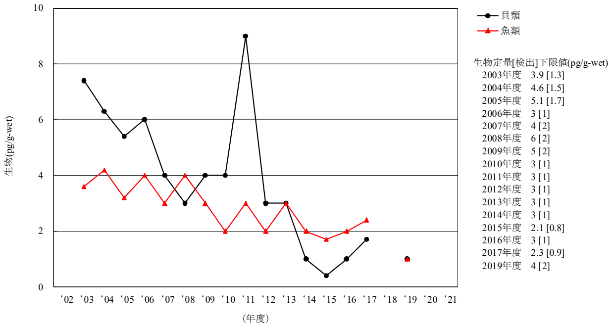
[11-4] δ-HCH
