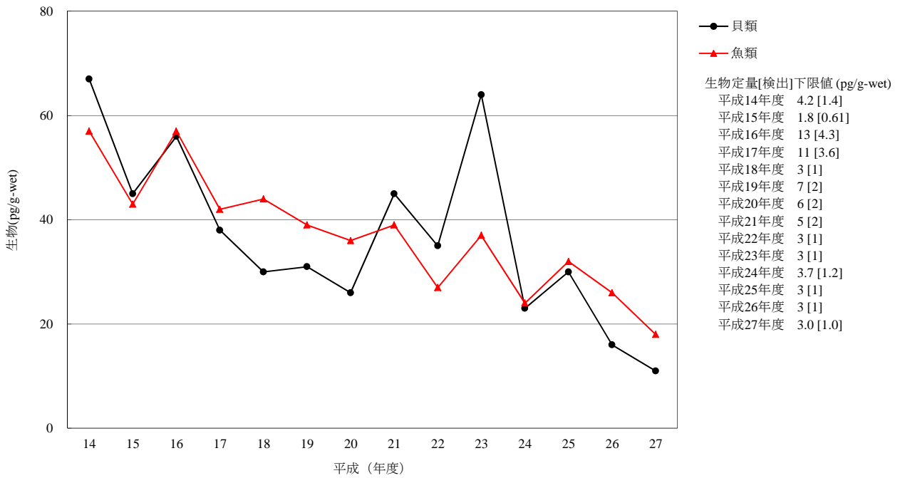
[11-1] \alpha -HCH
