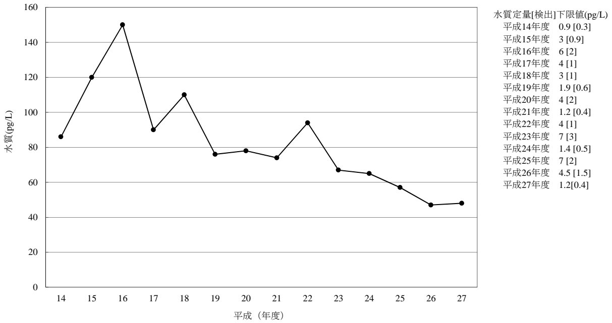
[11-1] \alpha -HCH
