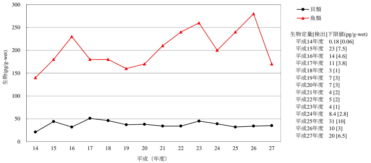
[2] HCB
