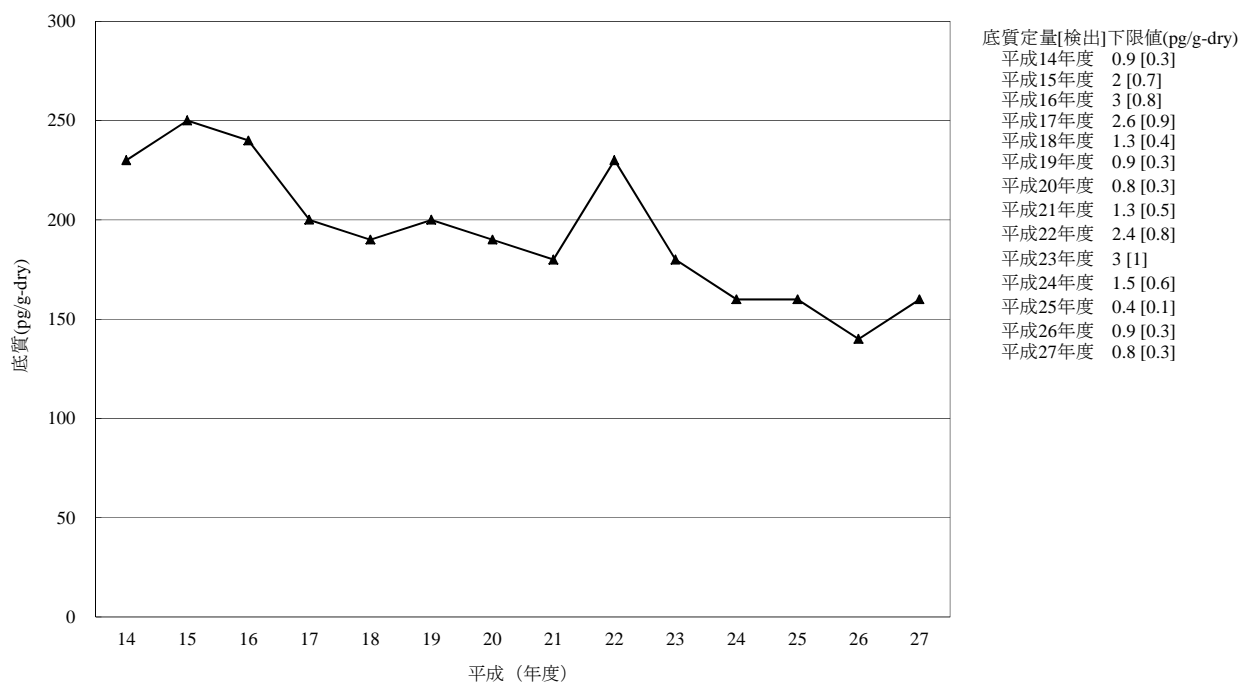
[11-2] \beta -HCH
