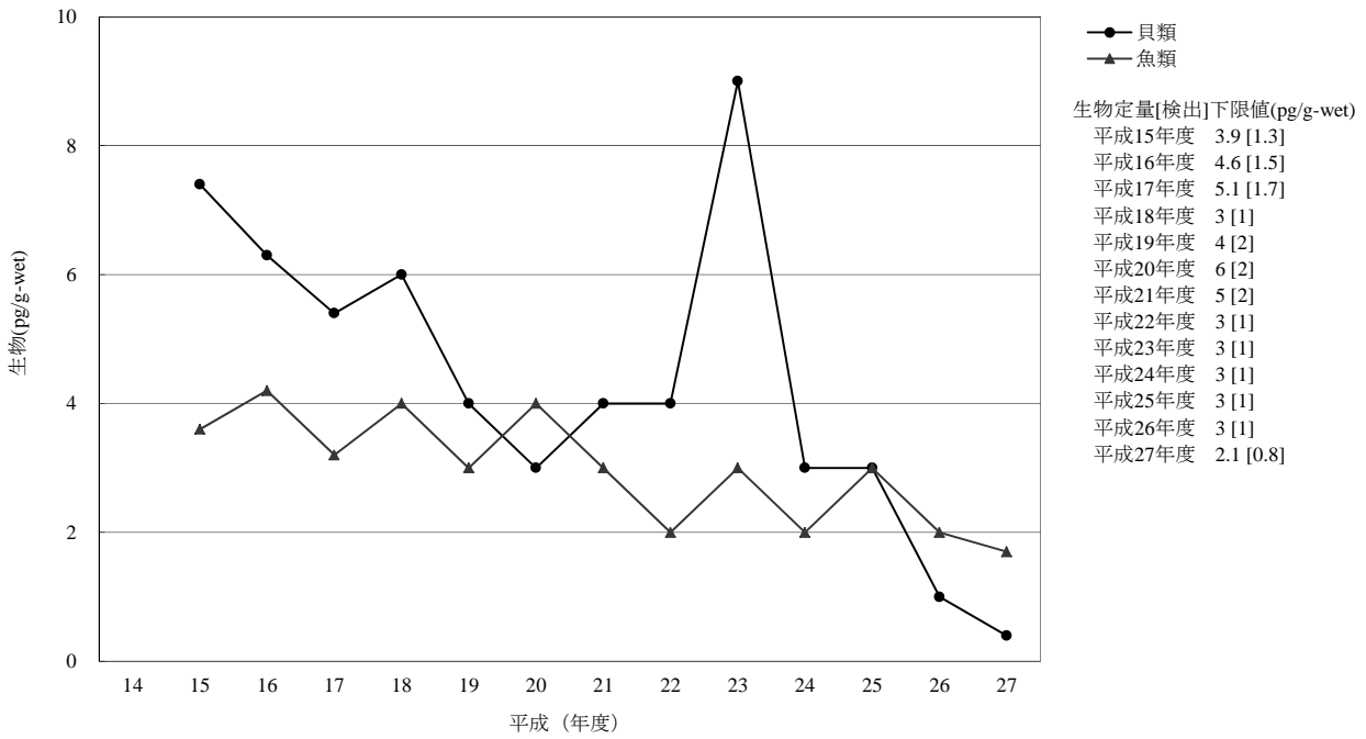
[11-4] δ-HCH
