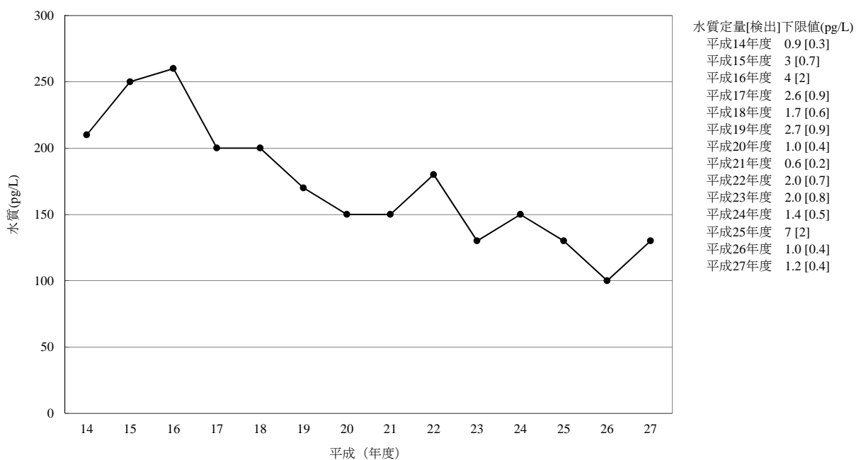
[11-2] \beta -HCH
