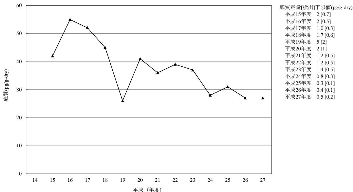
[11-4] δ-HCH
