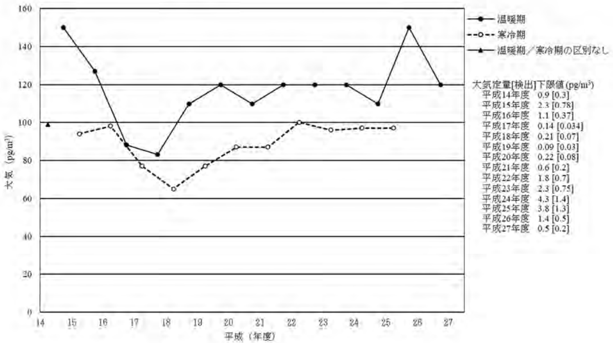
[2] HCB
