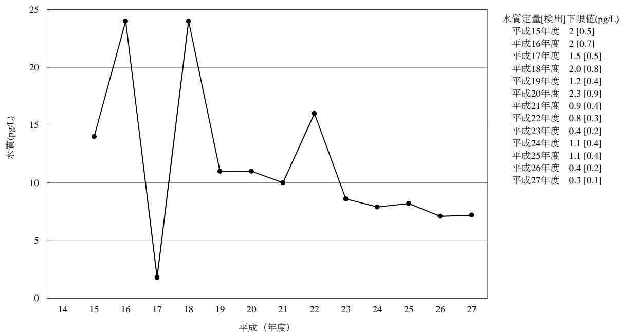
[11-4] δ-HCH
