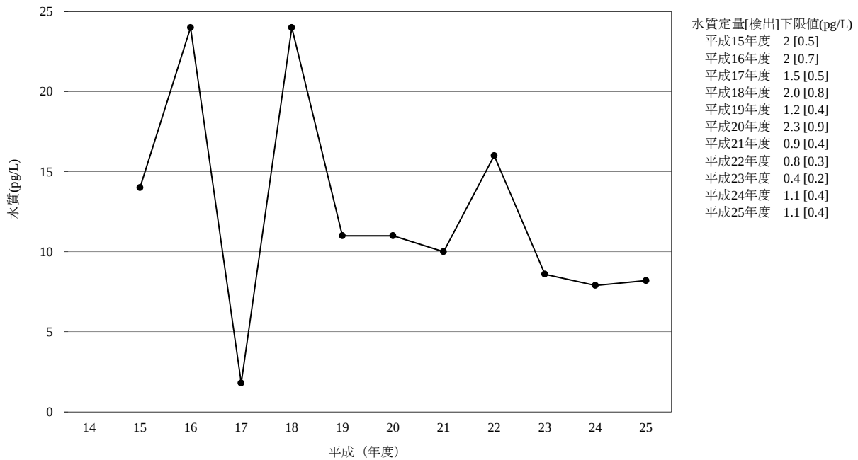
[11-4] \delta -HCH
