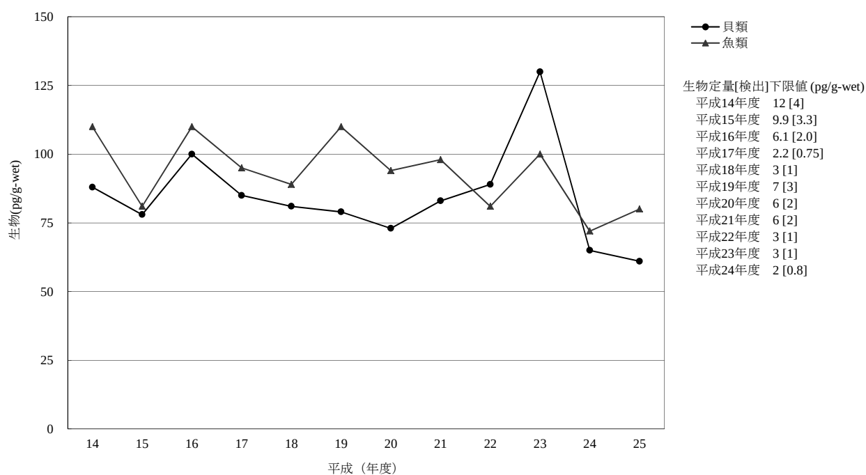
[11-2] \beta -HCH
