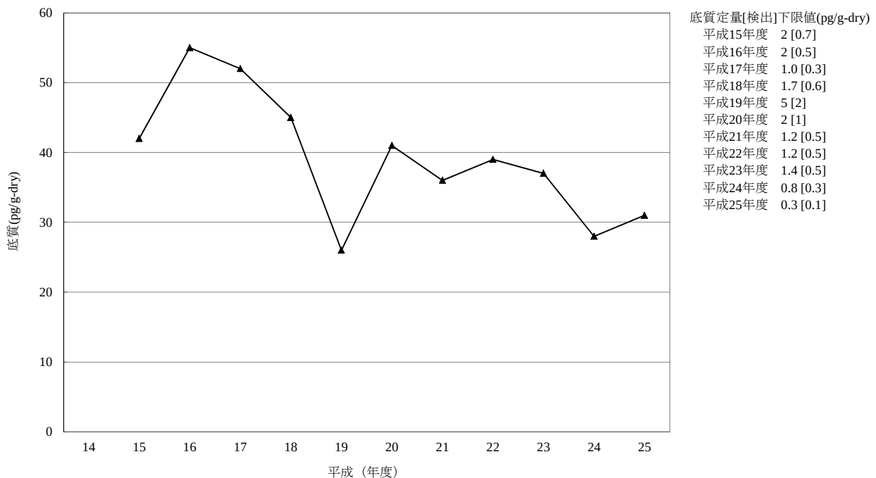
[11-4] \delta -HCH
