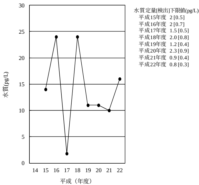
[11-4] \delta -HCH
