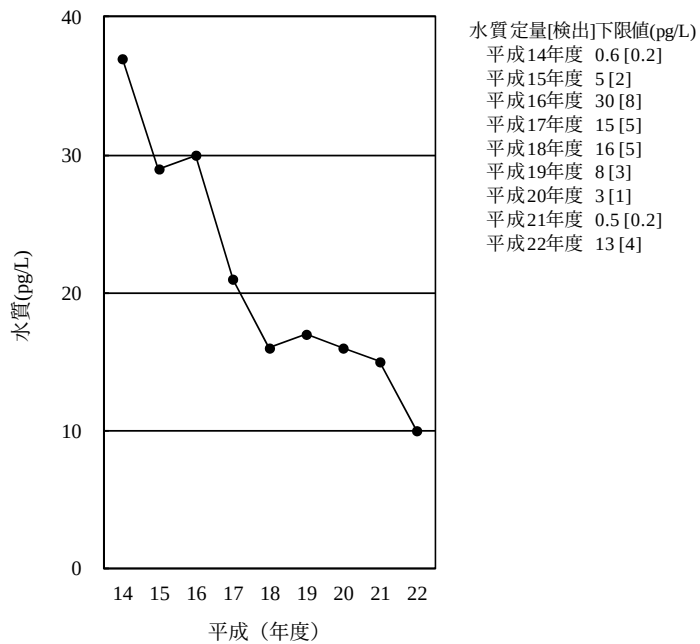
[2] HCB
