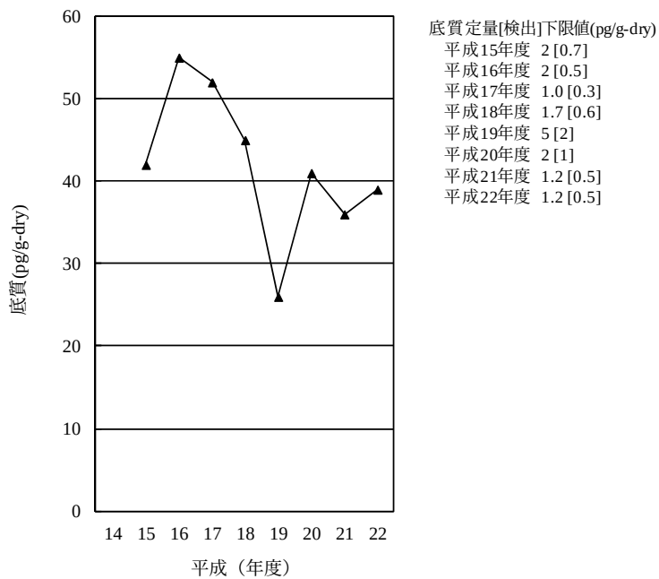
[11-4] \delta -HCH
