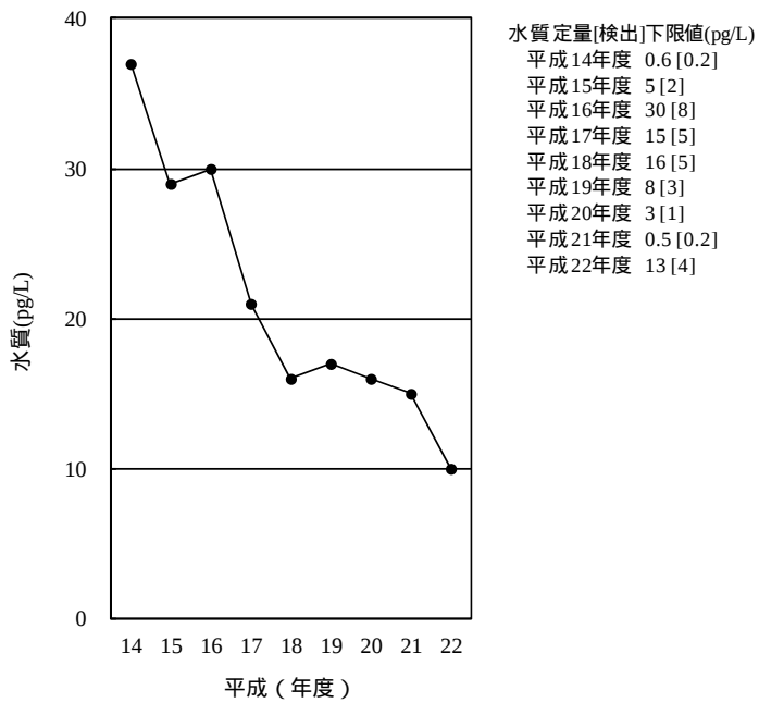
[2] HCB
