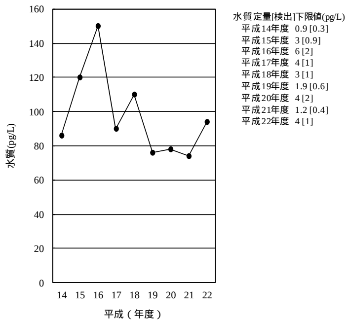
[11-1] \alpha -HCH
