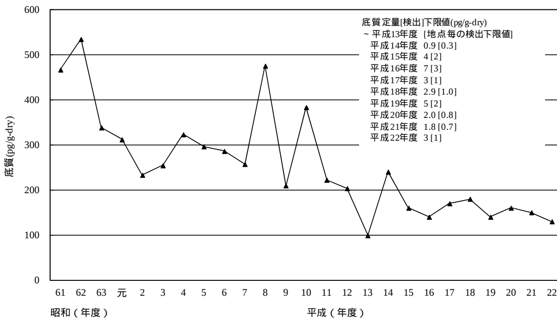
[2] HCB
