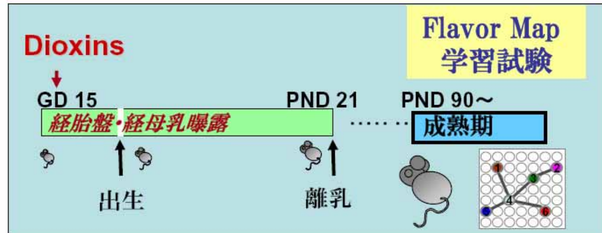
2,3,7,8-TBDD
