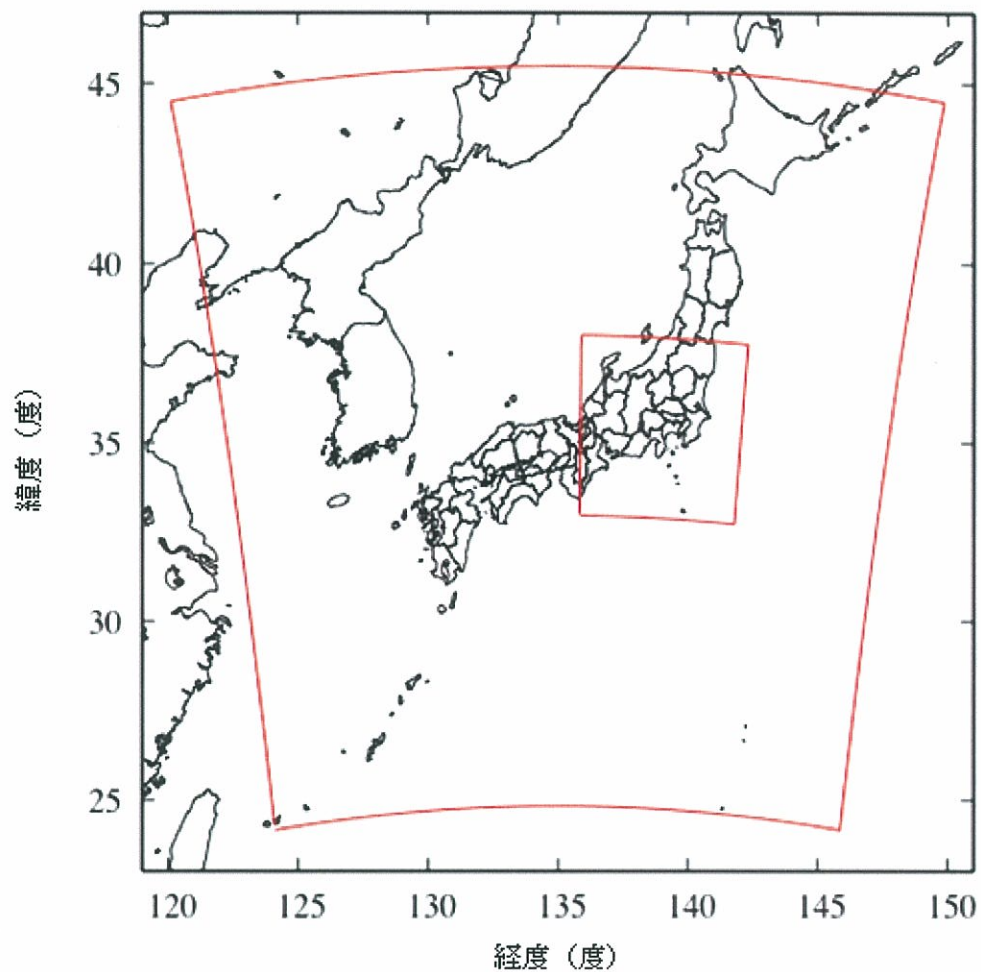
Model domains for WRF/Chem
