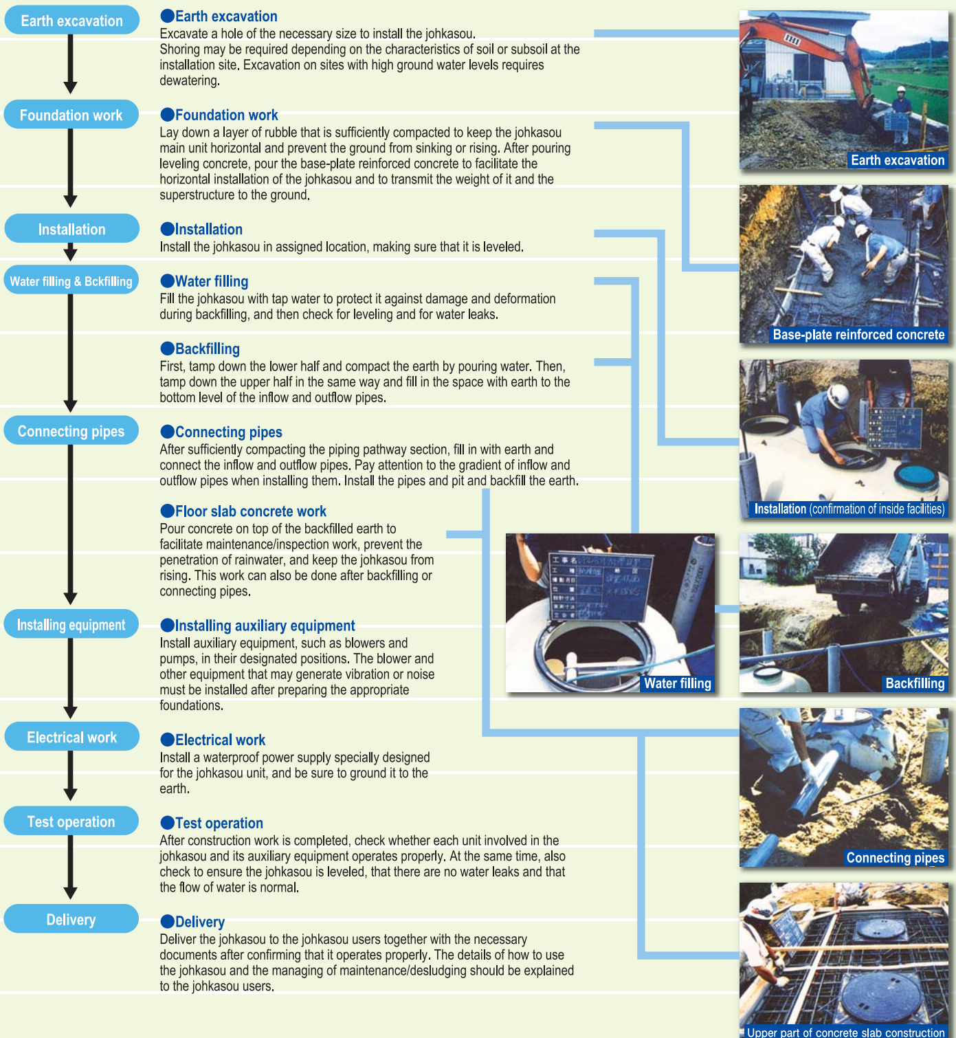
Figure 17 Construction procedure of a small-scale johkasou
