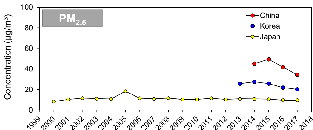
Fig. 2.6 Yearly mean concentrations of PM 2.5 in long-term monitoring period in China, Korea and Japan. Concentrations at the individual sampling sites were averaged.
