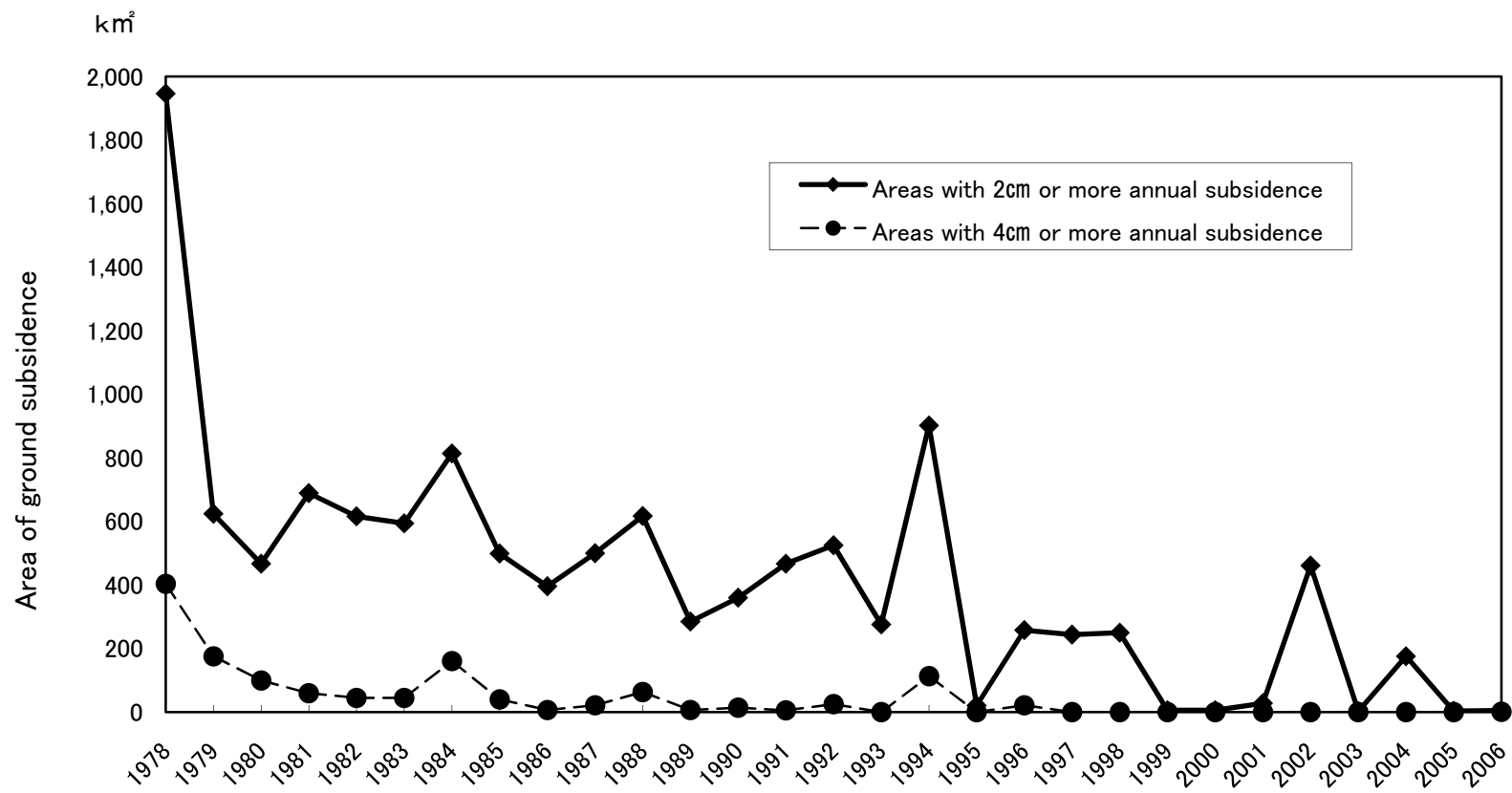
Fig. 2 Changes in Total Area of Ground Subsidence in Japan
