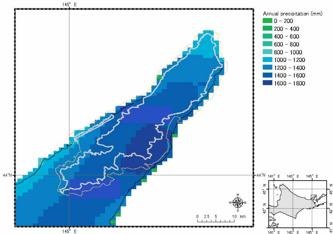
Figure 3-2 Annual precipitation (Japan Meteorological Agency, 2002)
